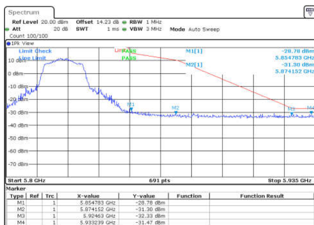
11AC40SISO-Ant1-5795-PASS
