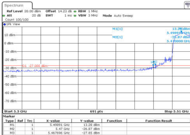
11AC40SISO-Ant1-5510-PASS
