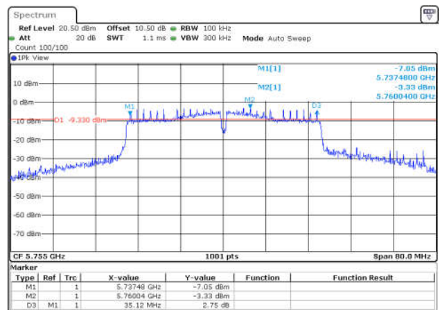
11AC40SISO-Ant1-5755-PASS
