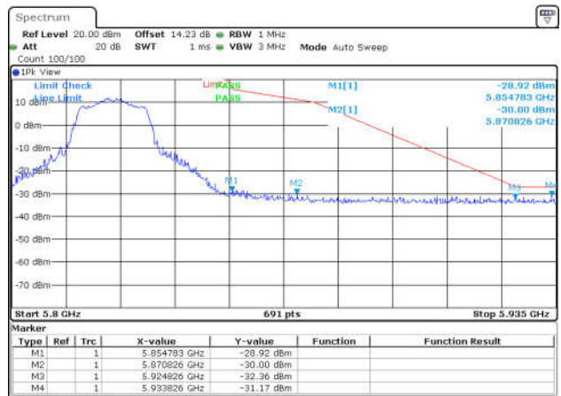
11N40SISO-Ant1-5795-PASS
