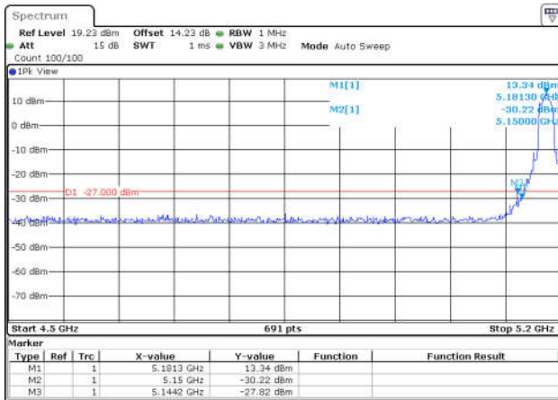
11AC40SISO-Ant1-5190-PASS
