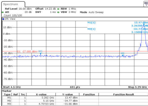
11AC40SISO-Ant1-5270-PASS
