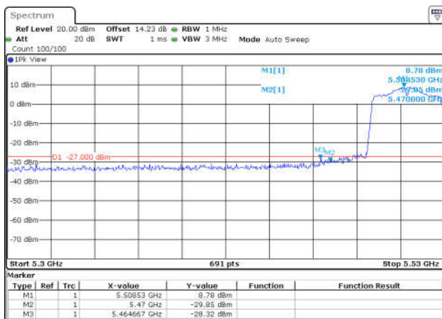
11N40SISO-Ant1-5510-PASS
