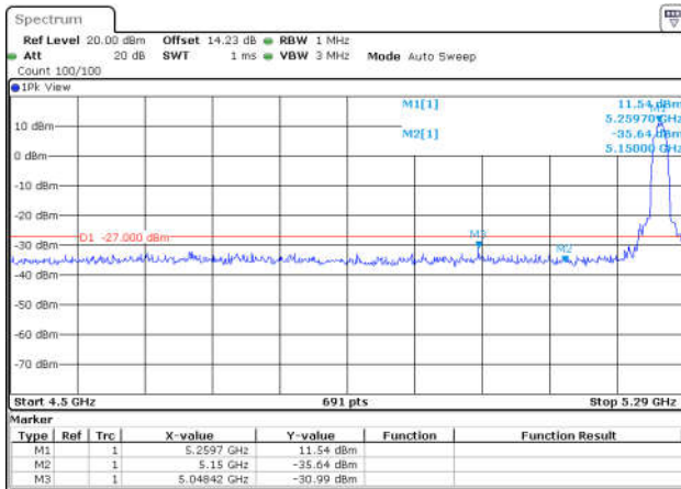
11N20SISO-Ant1-5260-PASS
