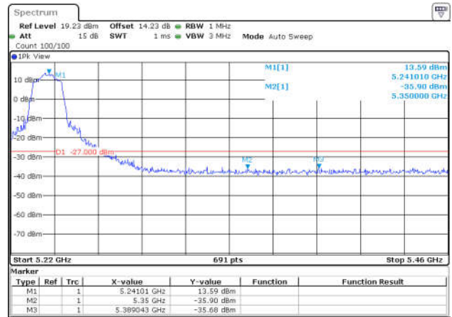
11N20SISO-Ant1-5240-PASS
