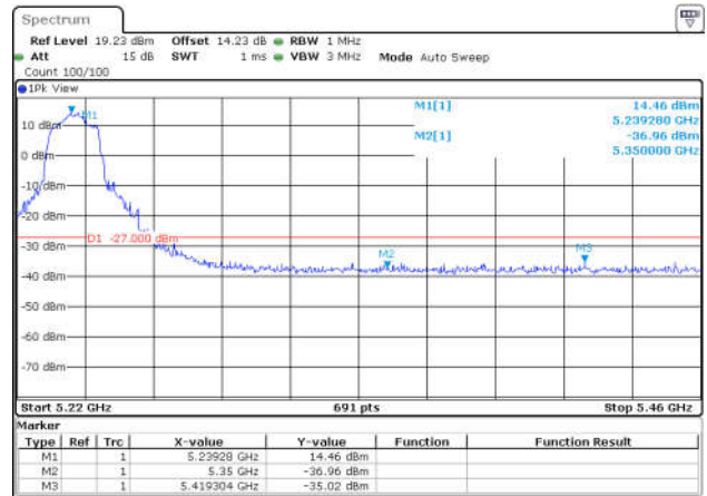
11AC40SISO-Ant1-5230-PASS
