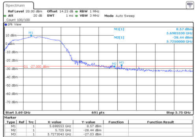
11N20SISO-Ant1-5700-PASS
