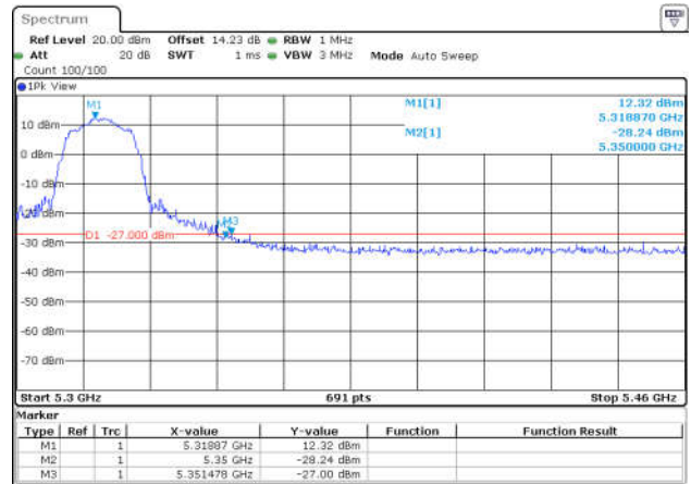
11N20SISO-Ant1-5320-PASS
