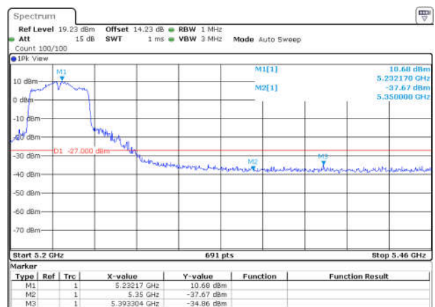
11N40SISO-Ant1-5230-PASS
