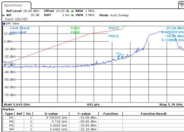
11N20SISO-Ant1-5745-PASS
