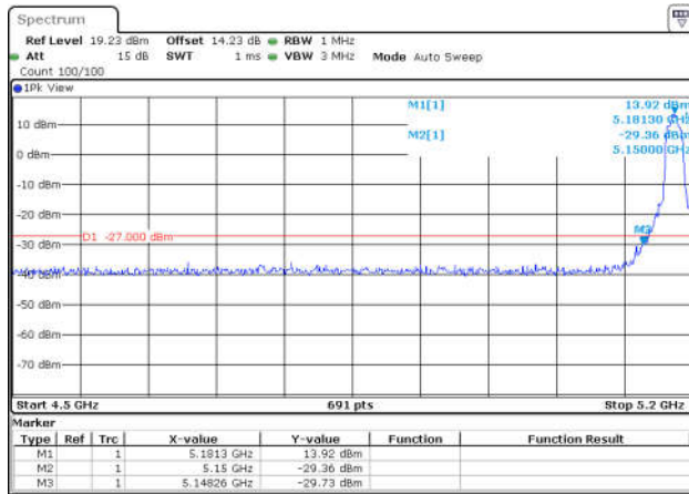
11N20SISO-Ant1-5180-PASS
