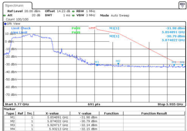
11N40SISO-Ant1-5795-PASS
