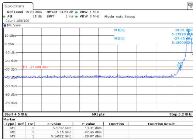
11N40SISO-Ant1-5190-PASS
