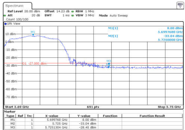
11N40SISO-Ant1-5670-PASS
