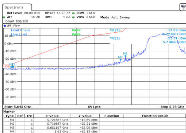
11AC40SISO-Ant1-5755-PASS
