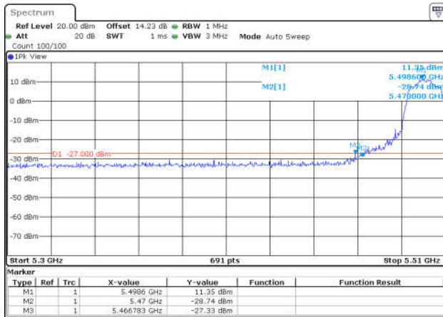
11N20SISO-Ant1-5500-PASS
