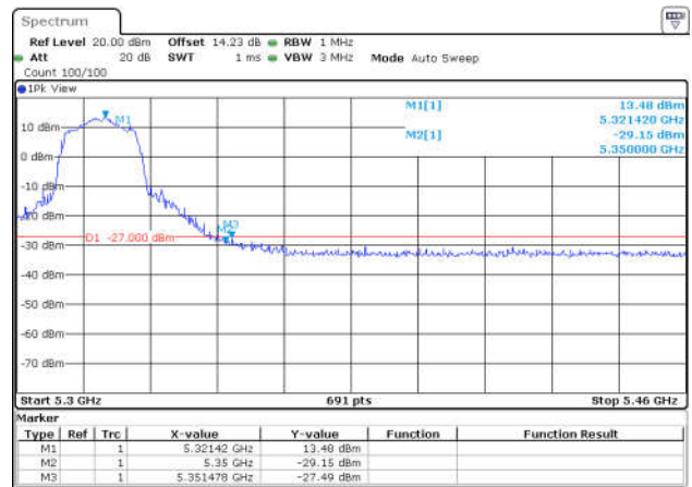
11N40SISO-Ant1-5310-PASS
