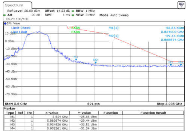
11N20SISO-Ant1-5825-PASS
