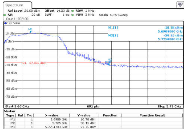
11AC40SISO-Ant1-5670-PASS
