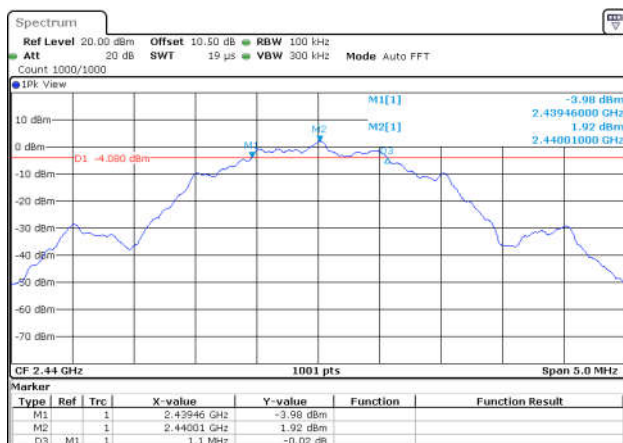
BLE_2M-Ant1-2440-PASS
