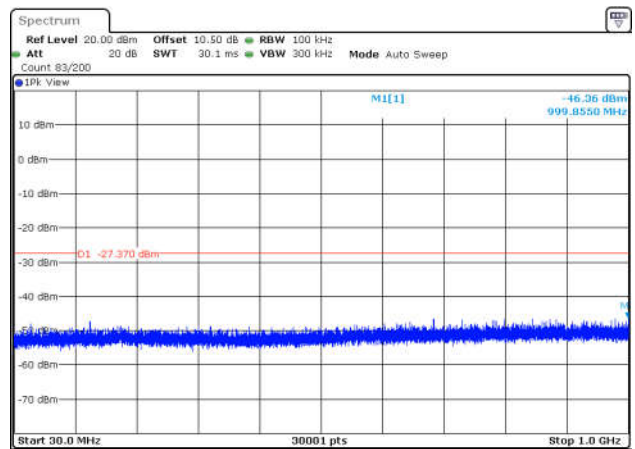
BLE_1M-Ant1-2440-0~Reference-PASS
