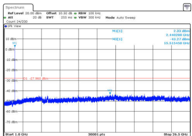
BLE_1M-Ant1-2440-1000~26500-PASS
