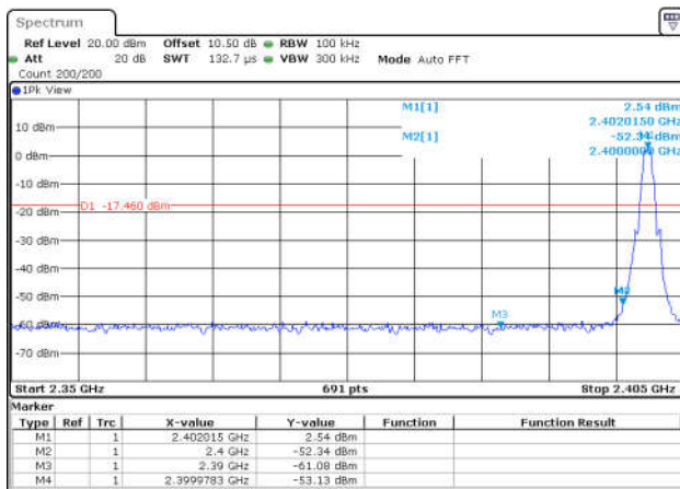
BLE_2M-Ant1-2402-PASS
