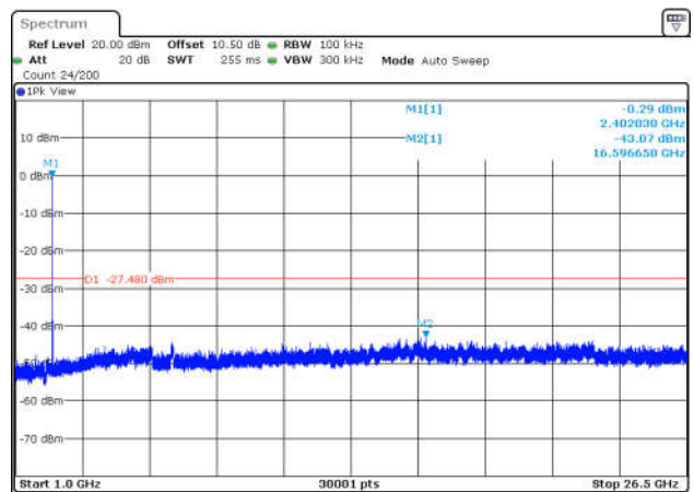
BLE_2M-Ant1-2402-1000~26500-PASS
