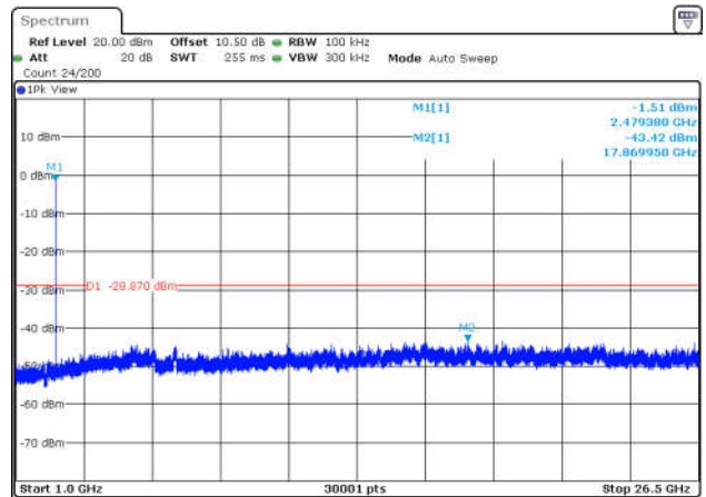
BLE_2M-Ant1-2480-1000~26500-PASS
