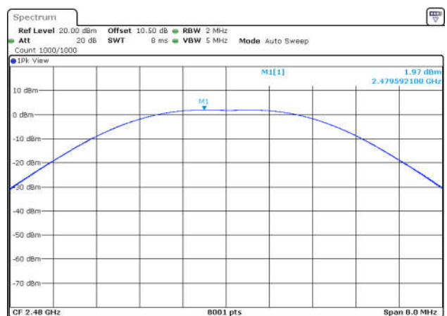
BLE_2M-Ant1-2480-PASS
