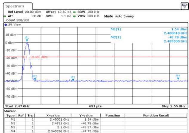
BLE_2M-Ant1-2480-PASS
