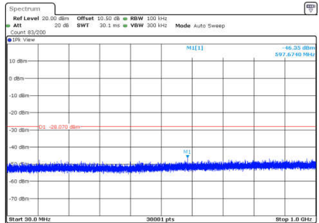
BLE_2M-Ant1-2480-0~Reference-PASS
