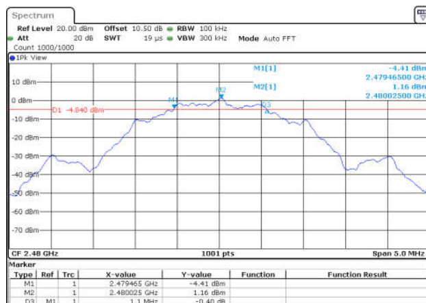
BLE_2M-Ant1-2480-PASS
