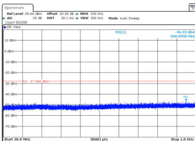
BLE_1M-Ant1-2440-30~1000-PASS
