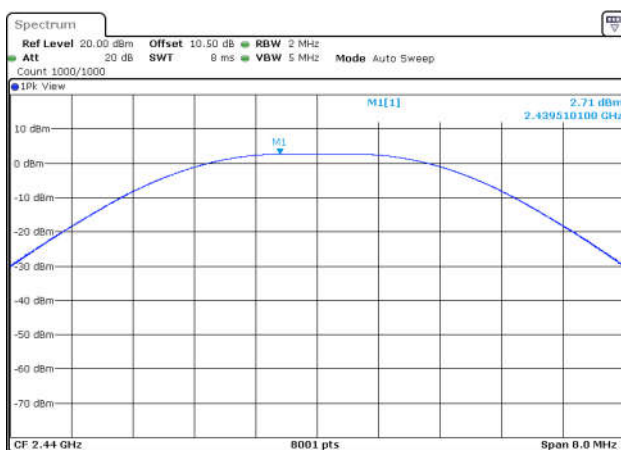
BLE_2M-Ant1-2440-PASS
