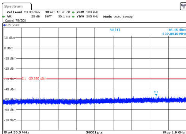
2DH5-Ant1-2480-30~1000-PASS
