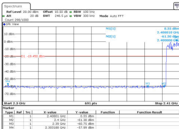
3DH5-Ant1-Hop_2402-PASS
