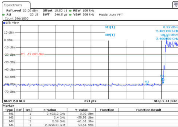
3DH5-Ant1-2402-PASS
