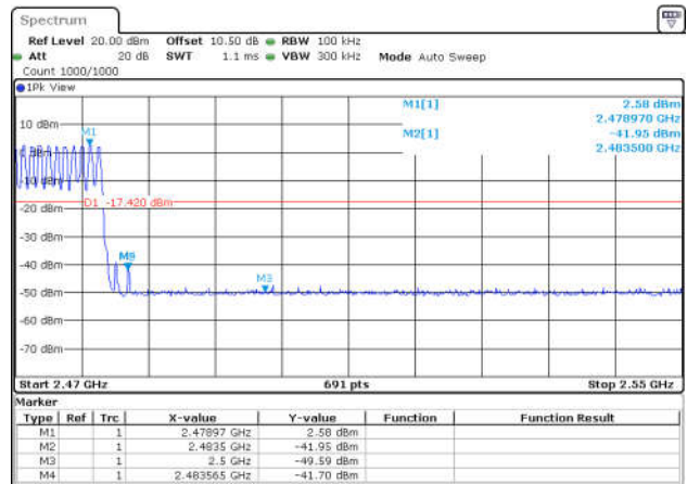
2DH5-Ant1-2480-PASS
