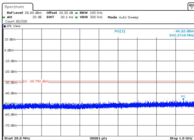
3DH5-Ant1-2441-30~1000-PASS
