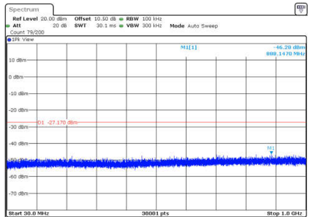
2DH5-Ant1-2402-0~Reference-PASS
