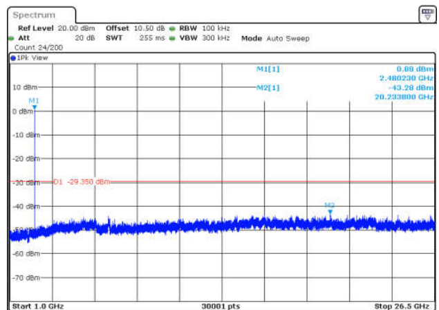
2DH5-Ant1-2480-1000~26500-PASS
