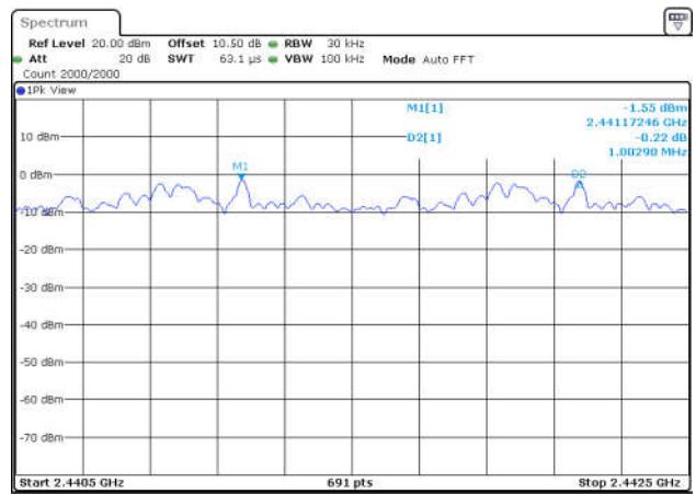
2DH5-Ant1-Hop-PASS
