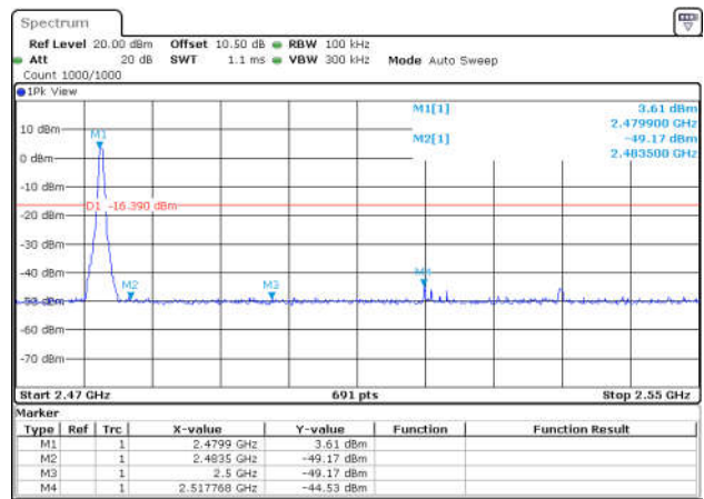
DH5-Ant1-Hop_2480-PASS
