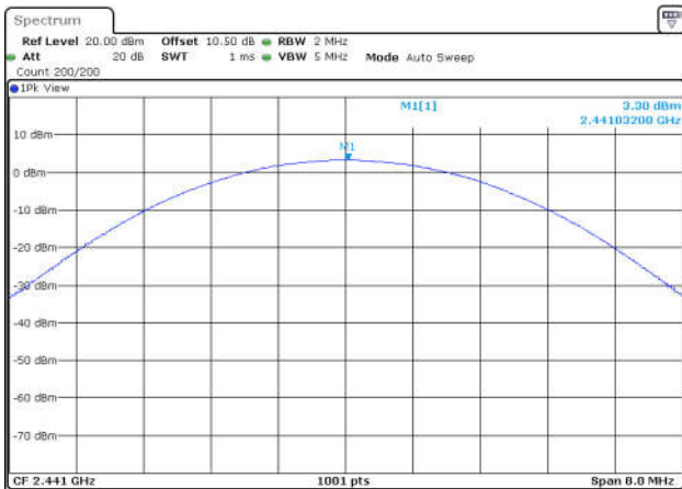
3DH5-Ant1-2441-PASS
