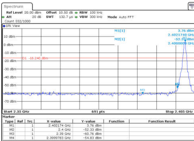
DH5-Ant1-Hop_2402-PASS
