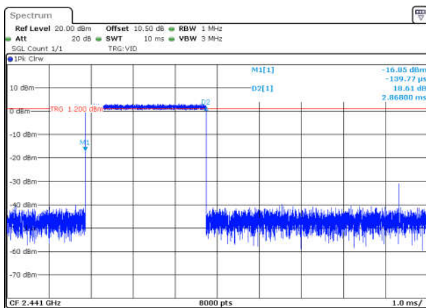
3DH5-Ant1-Hop-PASS
