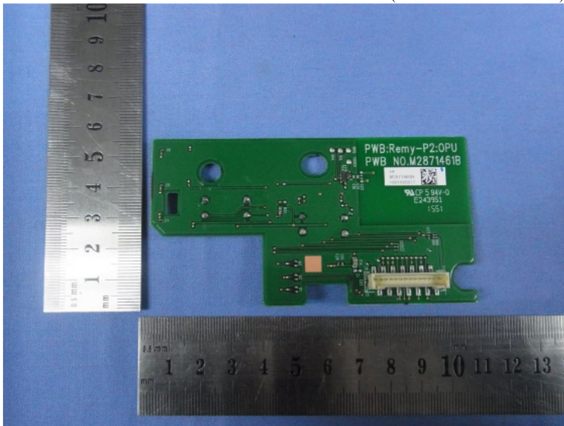
Figure 23 Internal View (Panel Board / Back View)
