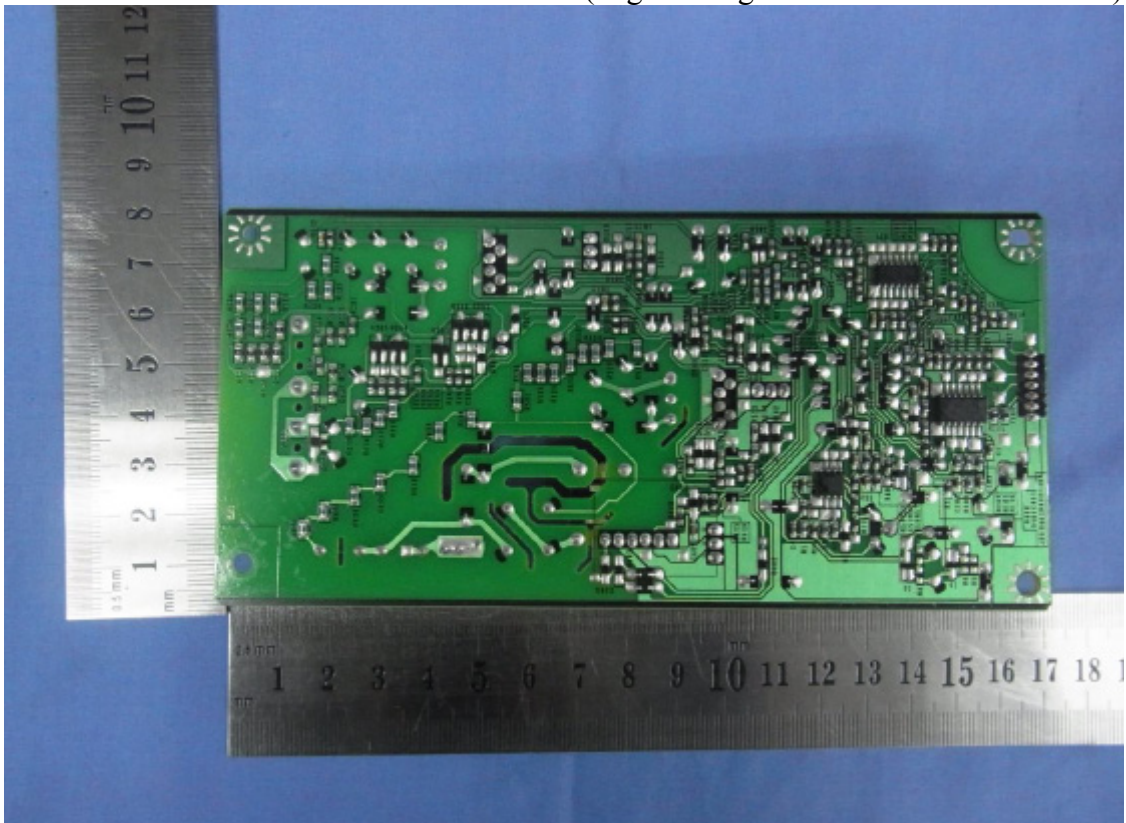
Figure 13 Internal View (High Voltage Power Board / Back View)
