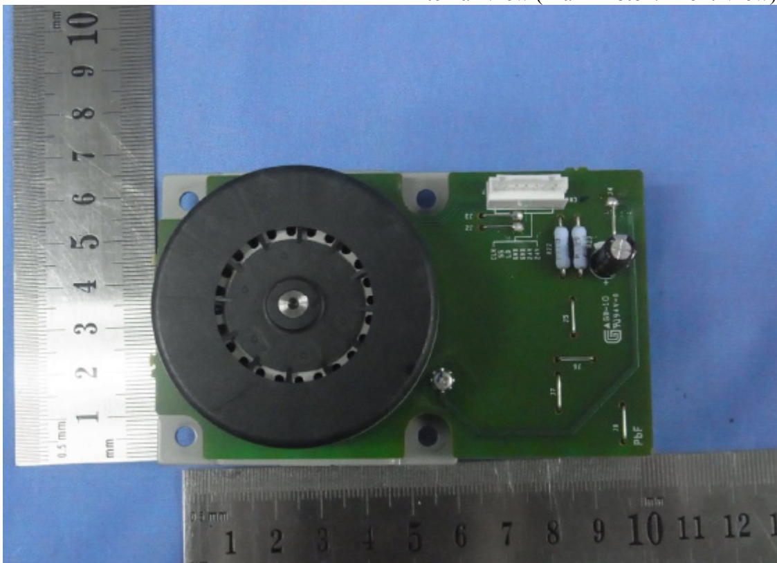
Figure 18 Internal View (Main Motor / Front View)
