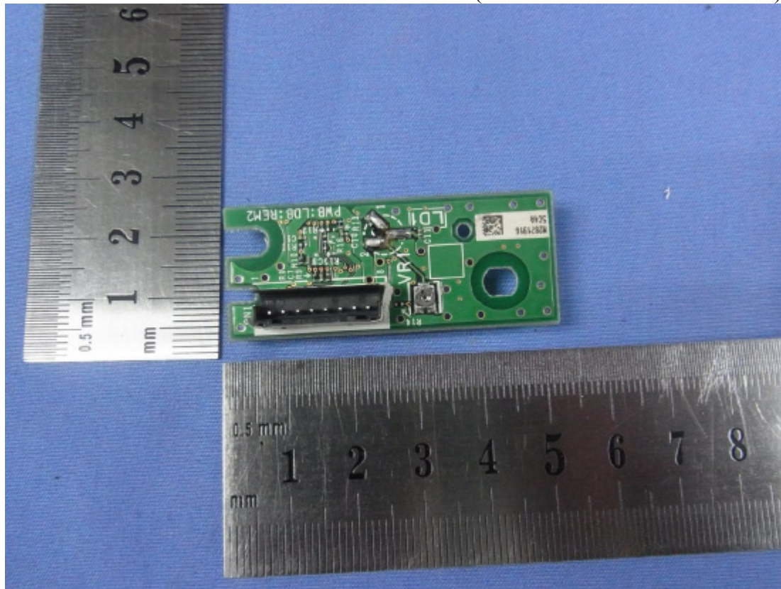
Figure 15 Internal View (Laser Diode Board / Back View)
