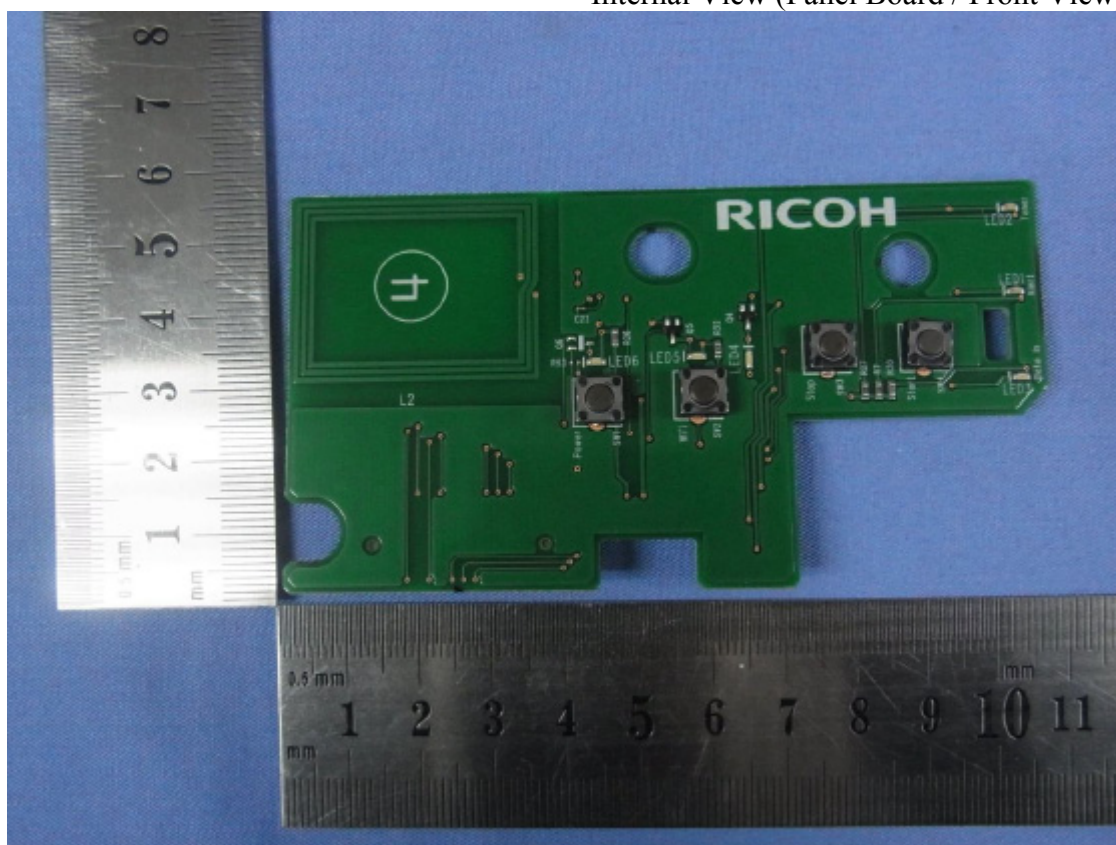
Figure 22 Internal View (Panel Board / Front View)
