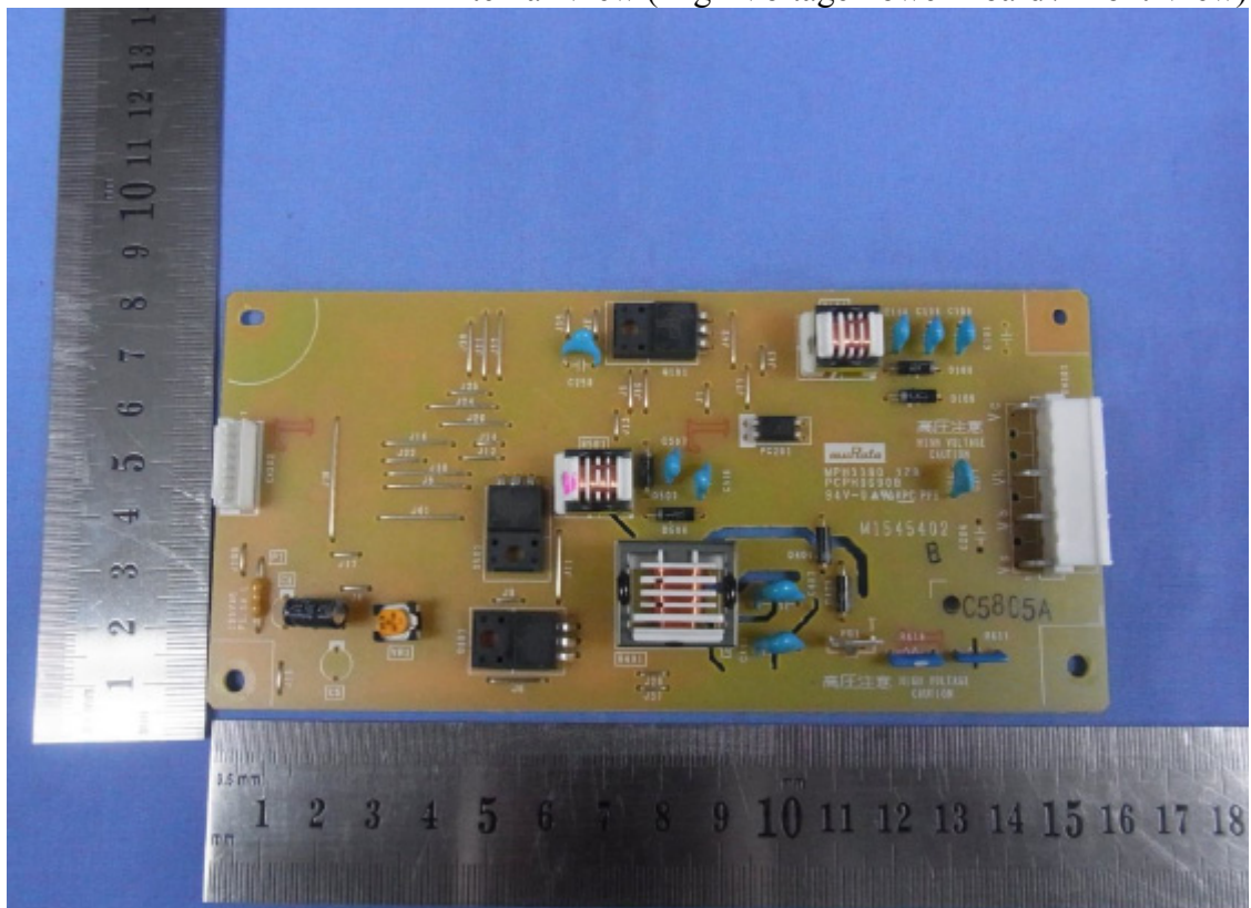
Figure 12 Internal View (High Voltage Power Board / Front View)
