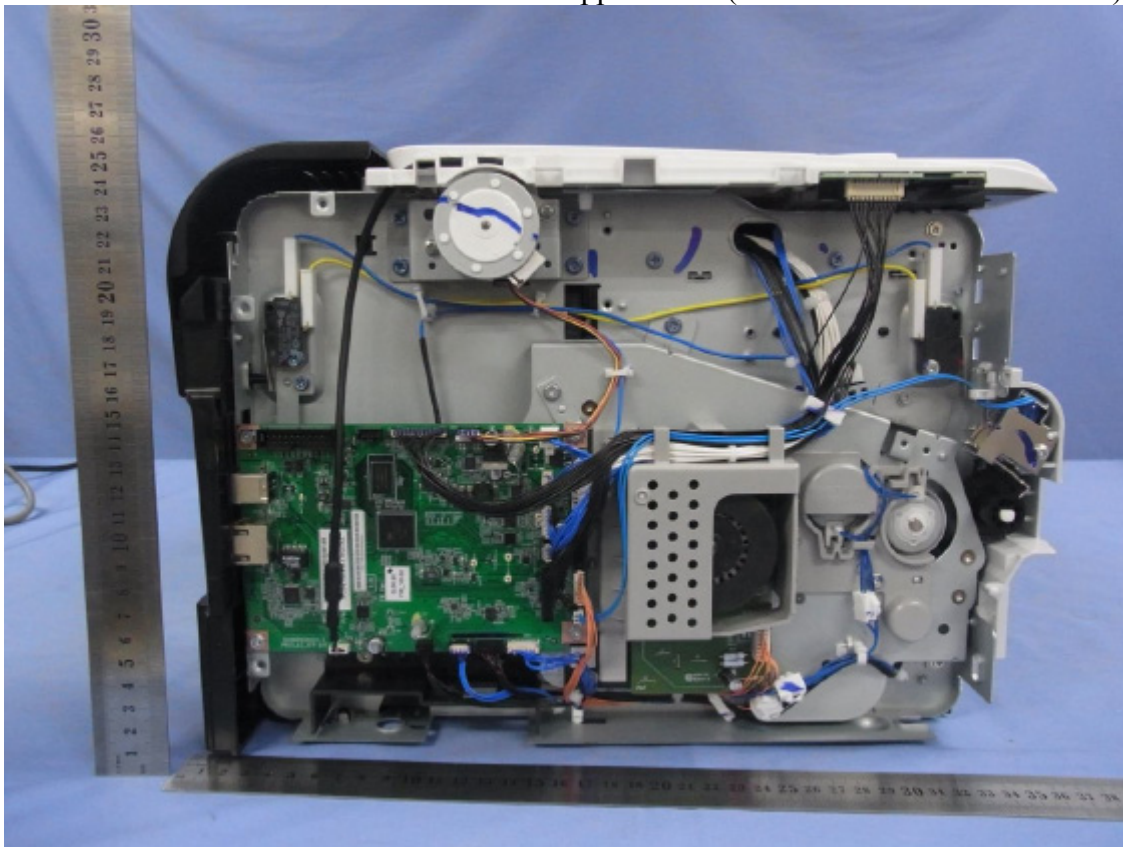
Figure 6 Appearance (Removed Side Cover View)
