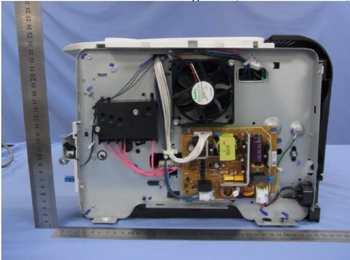
Figure 7 Appearance (Removed Side Cover View)
