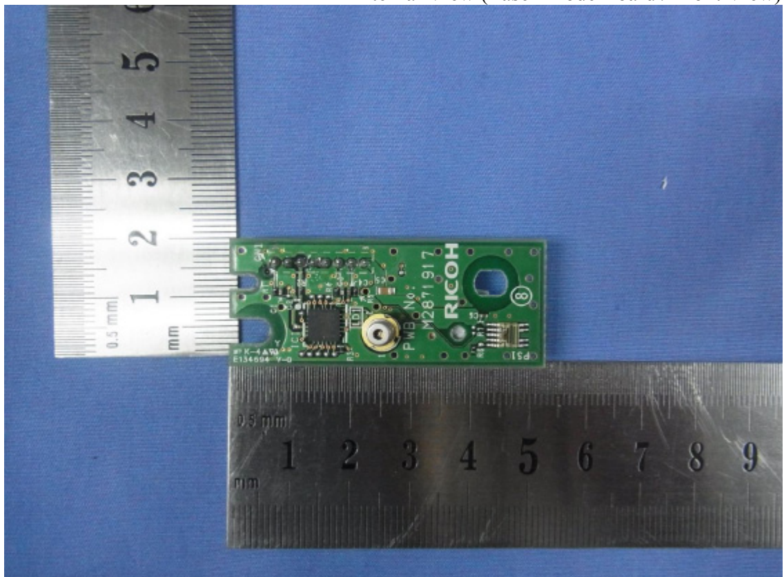
Figure 14 Internal View (Laser Diode Board / Front View)
