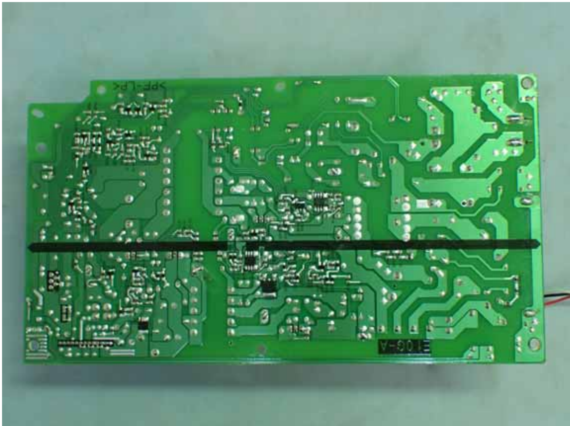
Figure 34 Internal View (Power Board, Back View)
