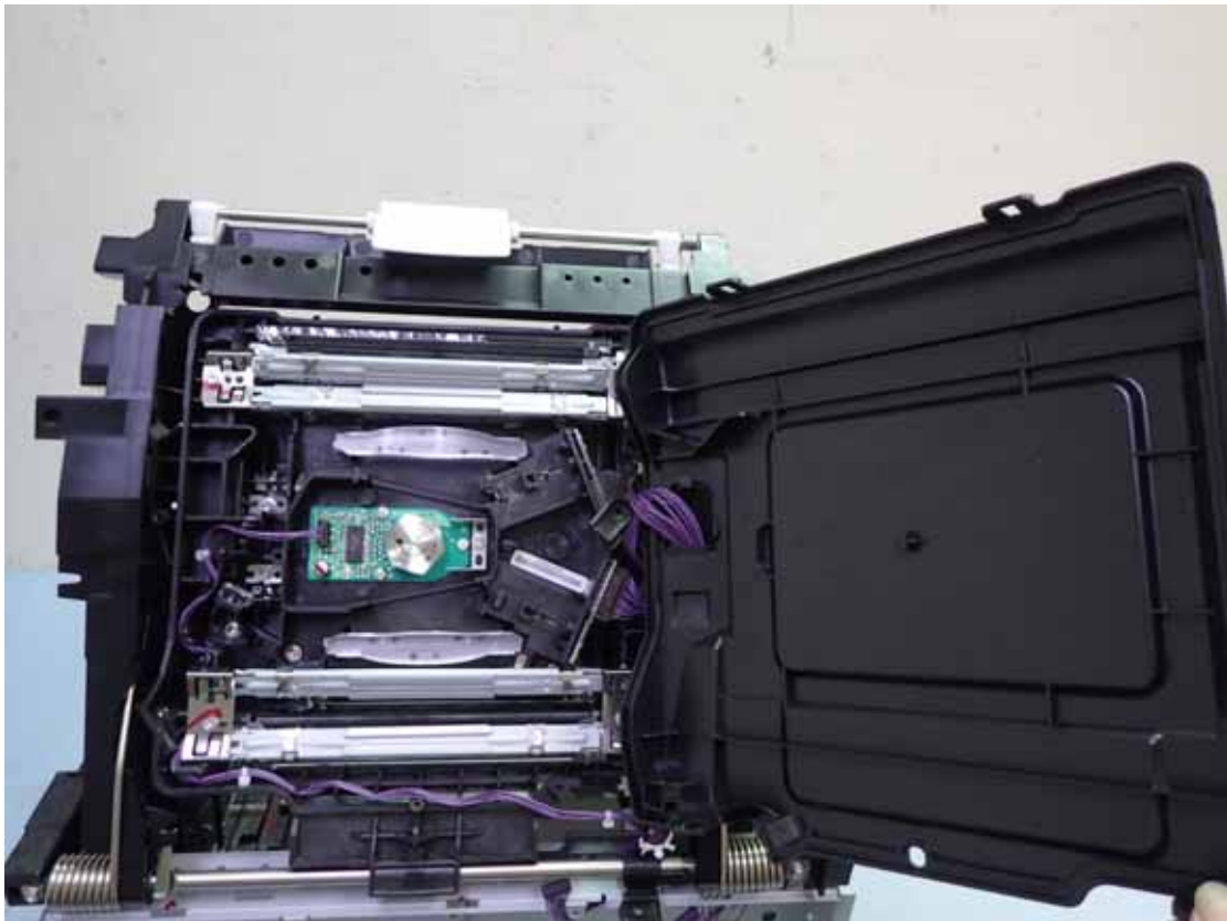
Figure 43 Internal View
