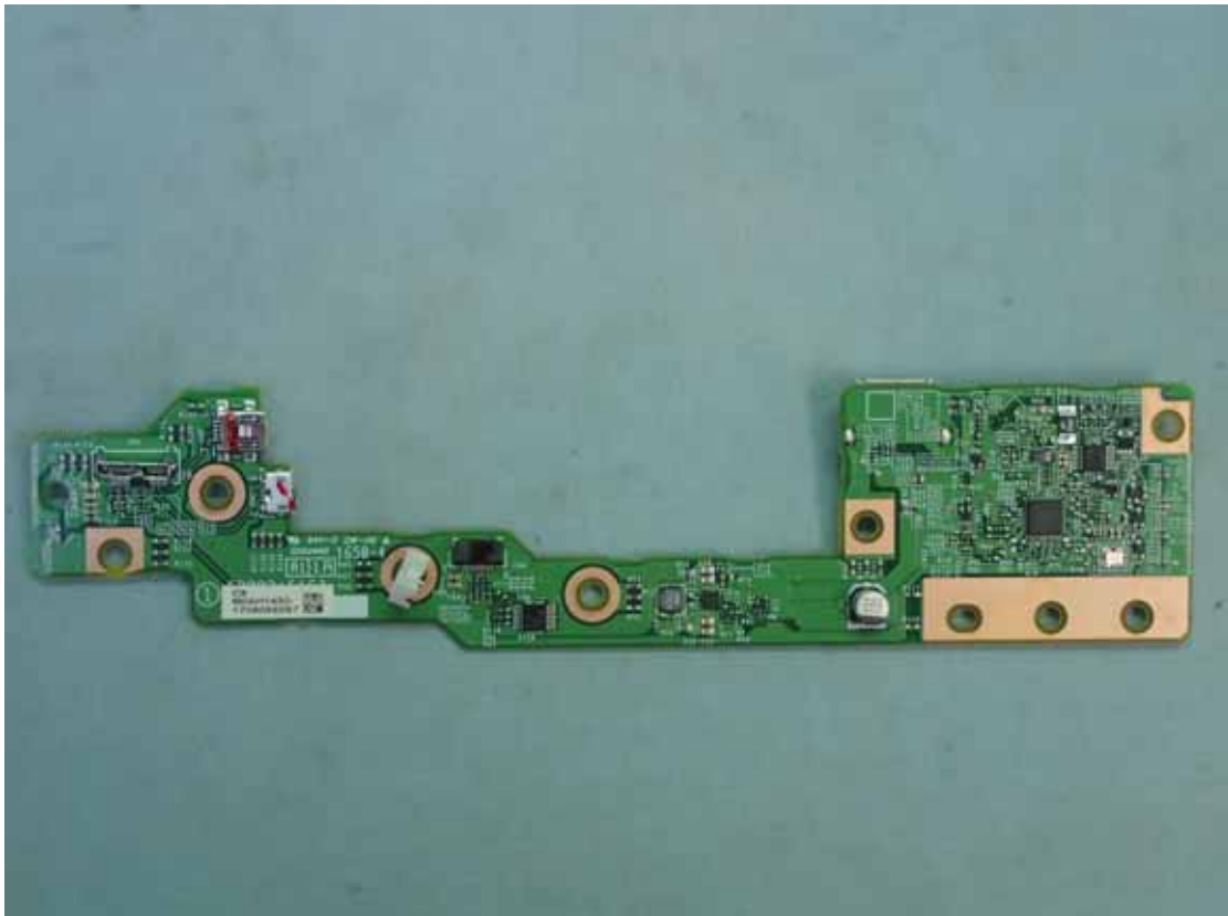
Figure 8 Internal View (Control Board, Front View)
