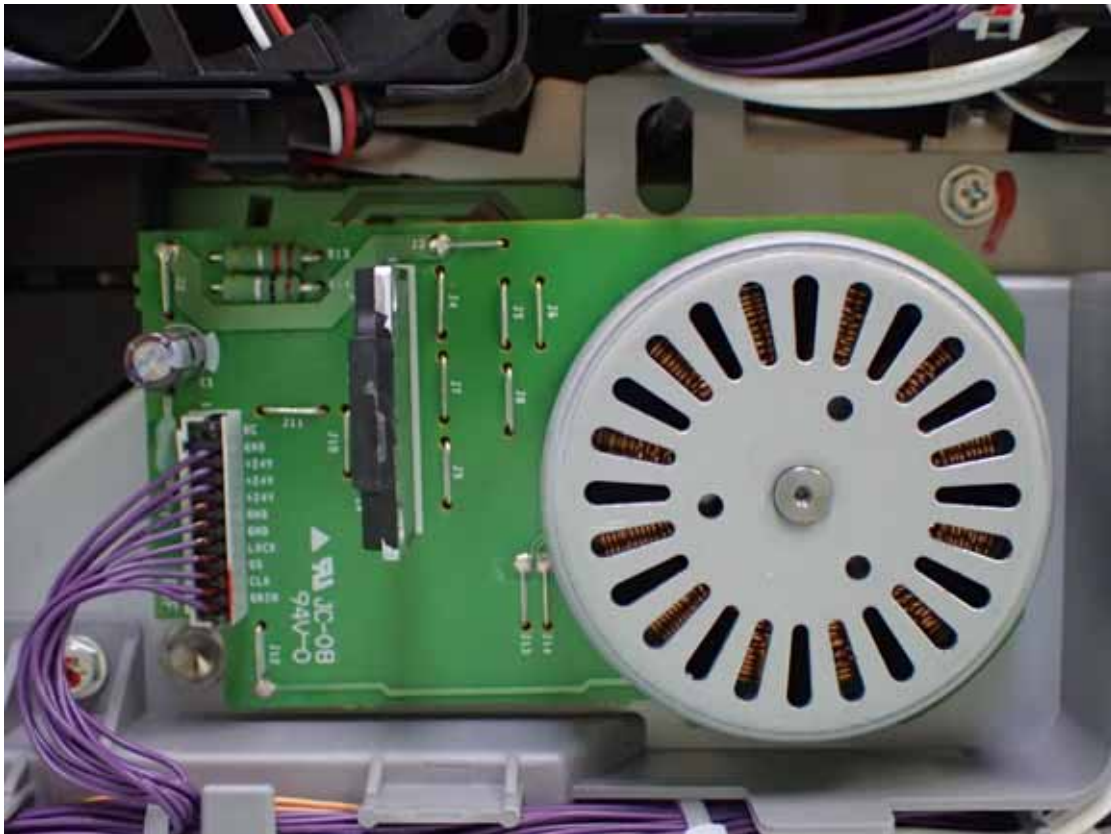
Figure 29 Internal View (Motor Board #1, Front View)
