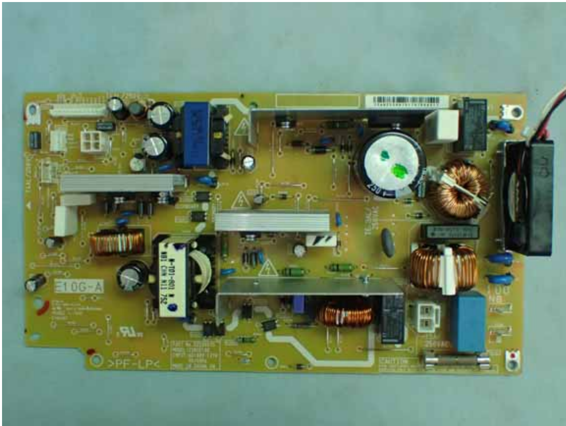
Figure 33 Internal View (Power Board, Front View)
