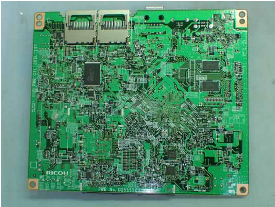
Figure 25 Internal View (Main Board #2, Back View)
