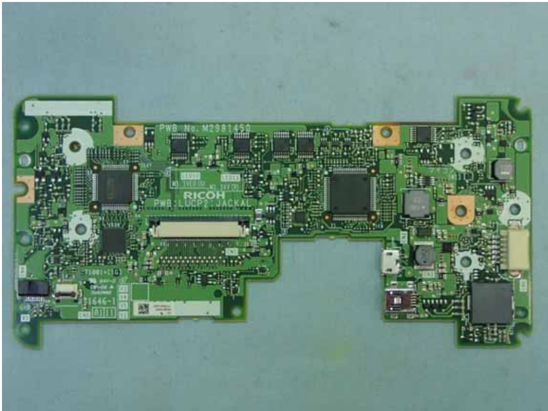
Figure 11 Internal View (Display Control Board, Front View)
