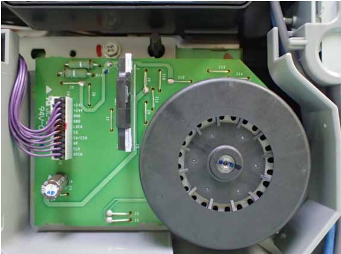
Figure 30 Internal View (Motor Board #2, Front View)
