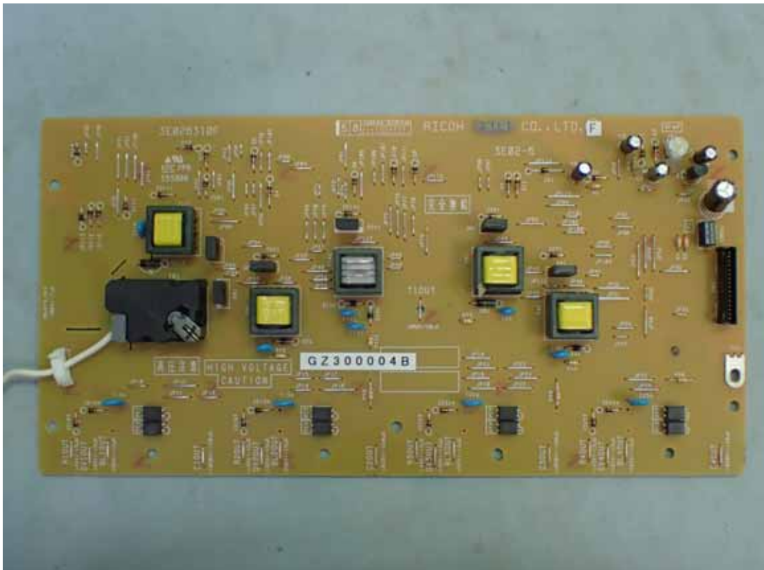
Figure 40 Internal View (HVPS Board, Front View)
