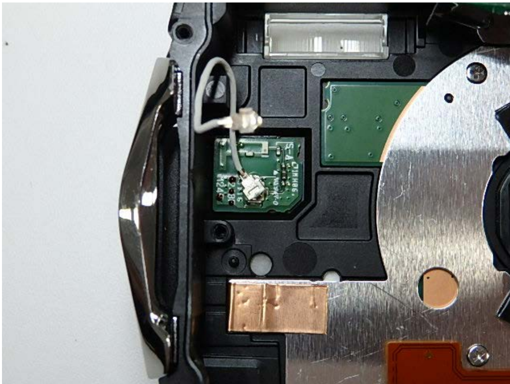
RF2 Board (BT&WLAN Antenna)
