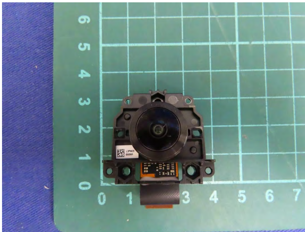
(38) EUT Photo
