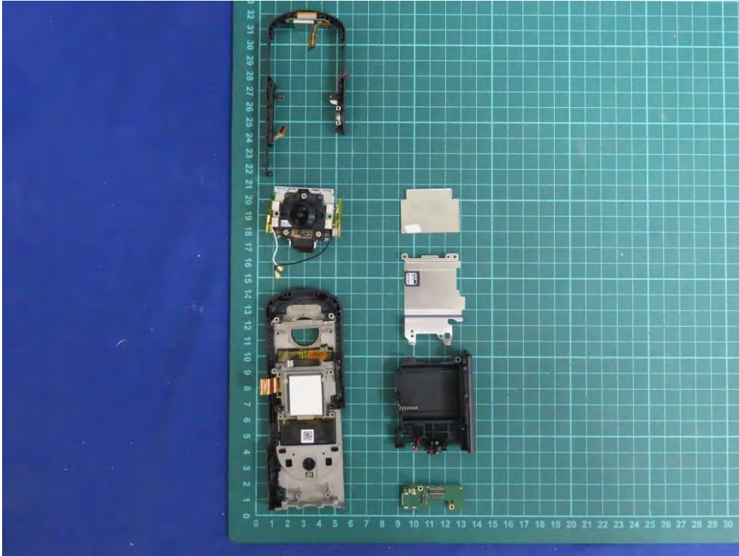
(22) EUT Photo
