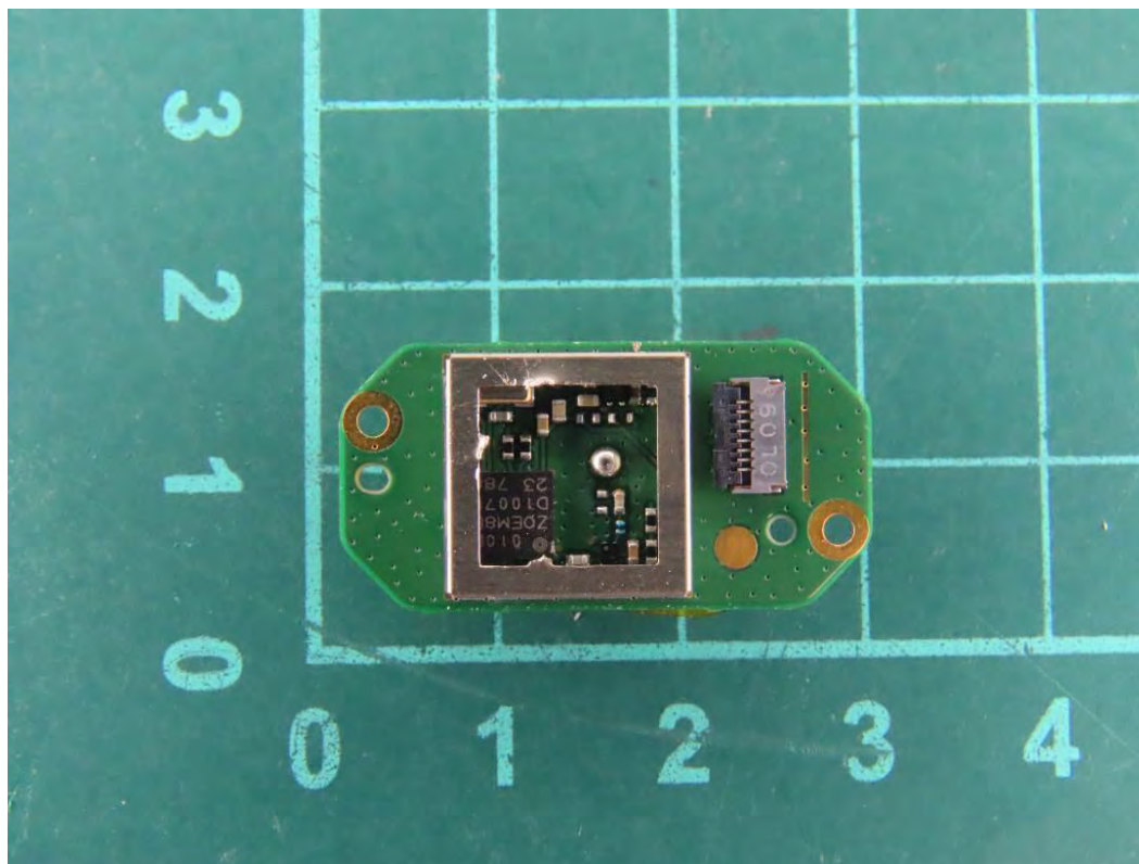
(28) EUT Photo
