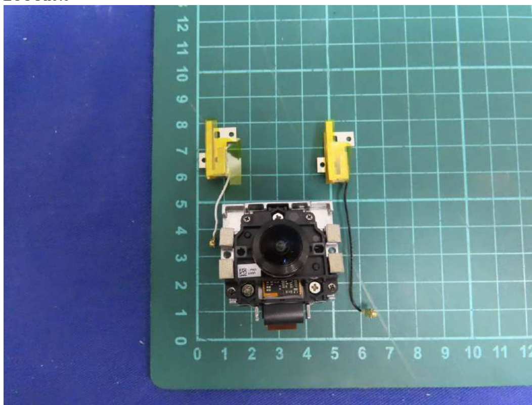
(38) EUT Photo
