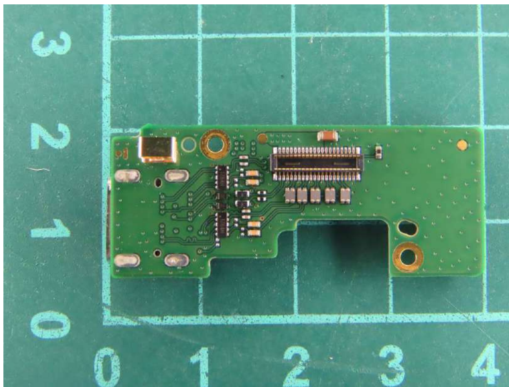
(51) EUT Photo
