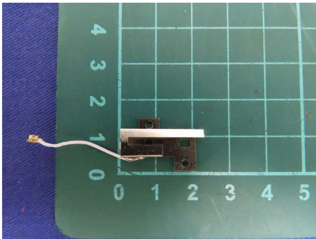
(39) EUT Photo
