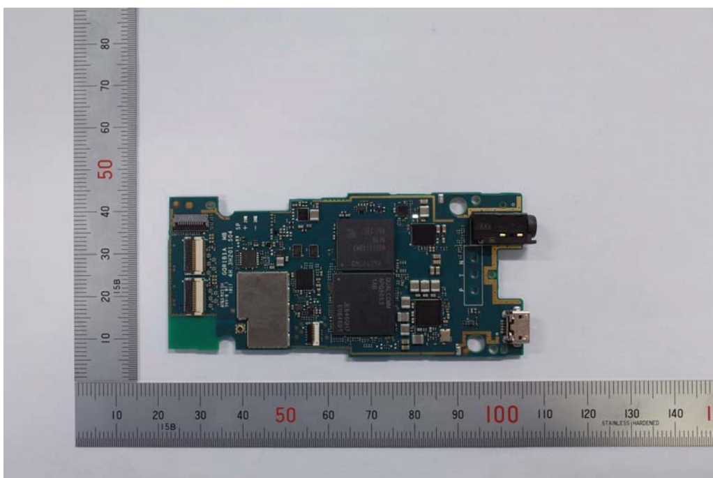
Lens Main PCB Back Side
