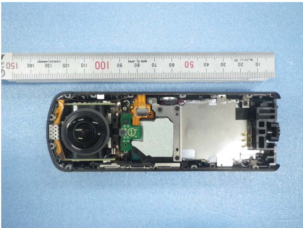
Front Cover Off With Out Battry
