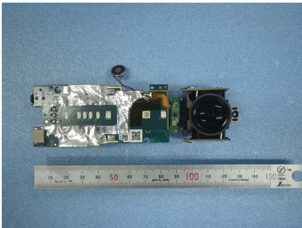
Lens Main PCB Back Side
