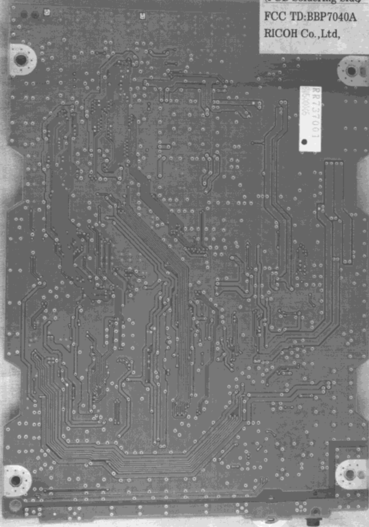
Fig.4 - Main PCB (PCB Soldering Side)
