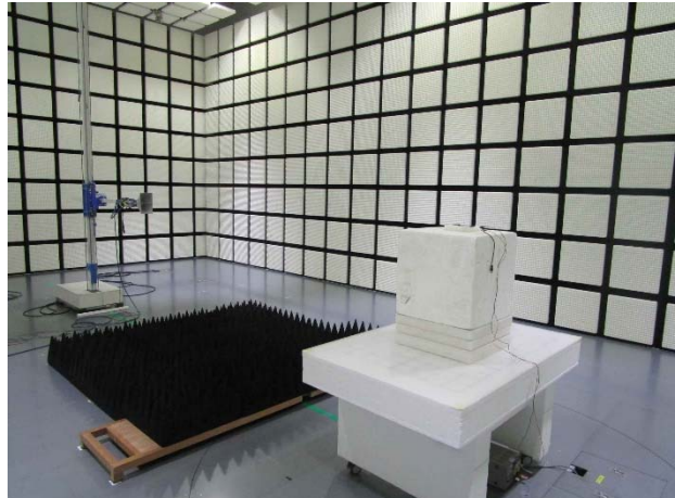
Above 1 GHz
