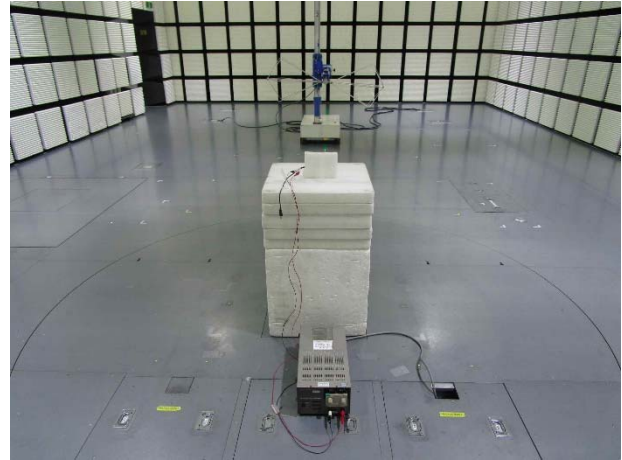
Below 1 GHz
