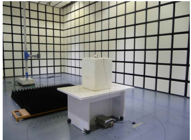
Above 1 GHz
