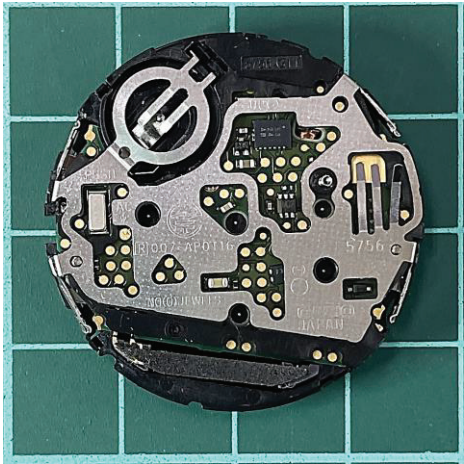
Watch Module Back
