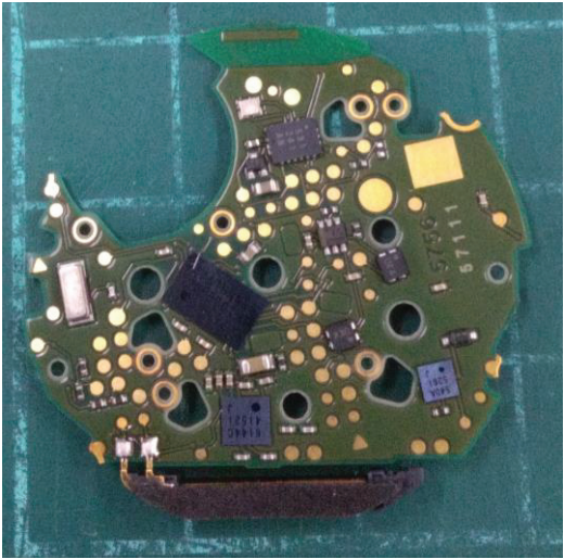
RF Module in Watch Module
