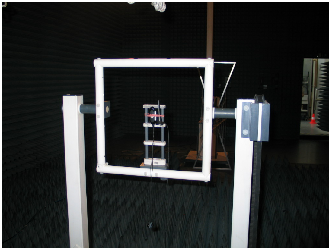
PHOTO No. 4: EUT (setup for radiated test)
