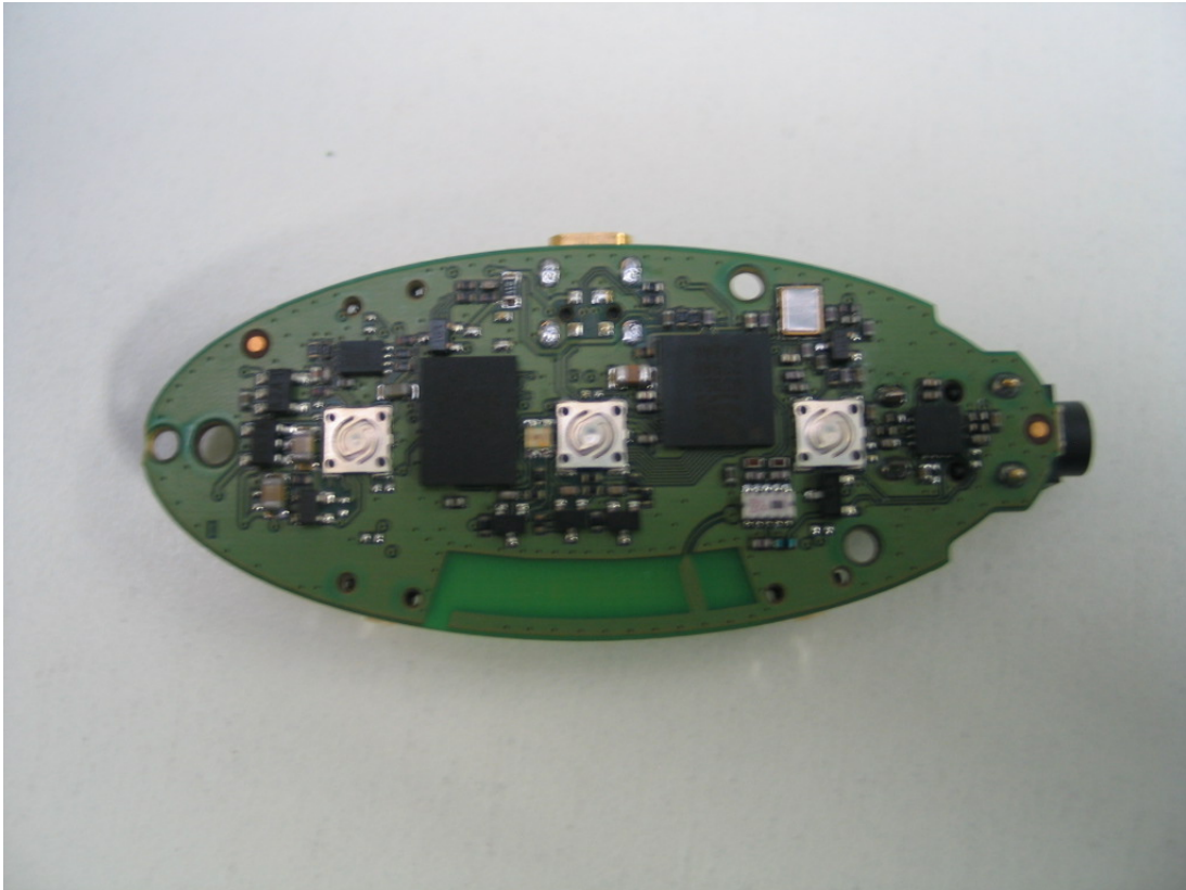
PHOTO No. 2: EUT without housing (top view)
