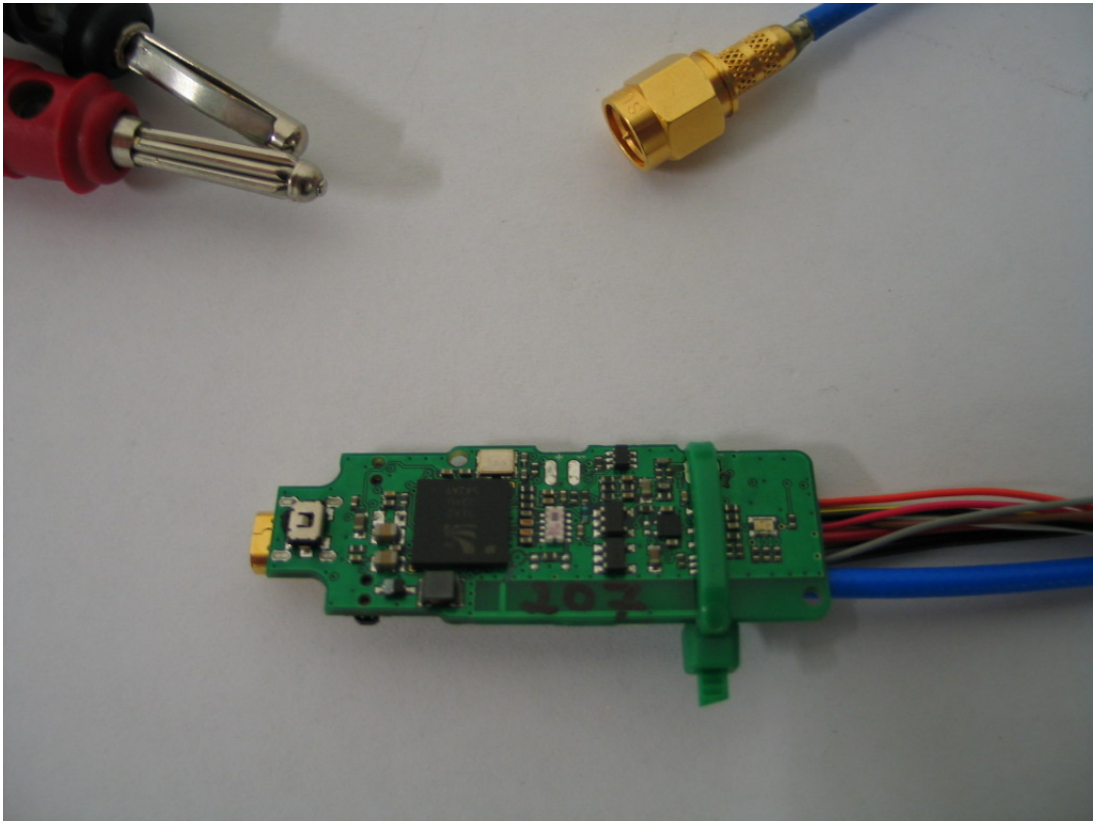
PHOTO No. 1: EUT, used for conducted measurements (top view) – without enclosure
