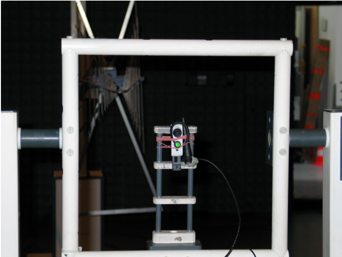
PHOTO No. 5: EUT, setup used for radiated measurements
