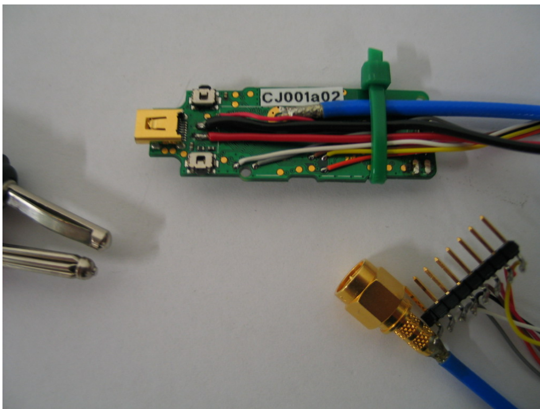
PHOTO No. 3: EUT, used for conducted measurements (bottom view) – without enclosure
