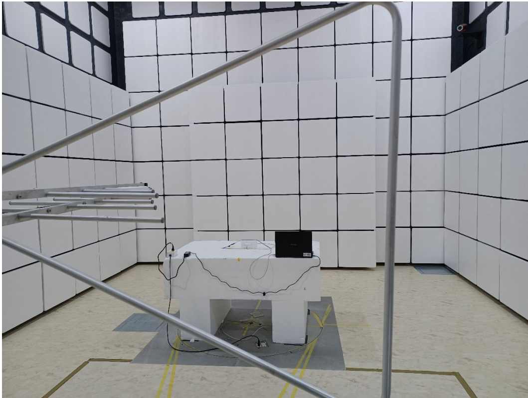
Radiated Test
