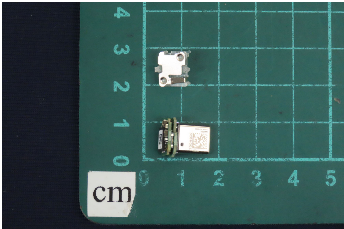
(11) EUT Photo
