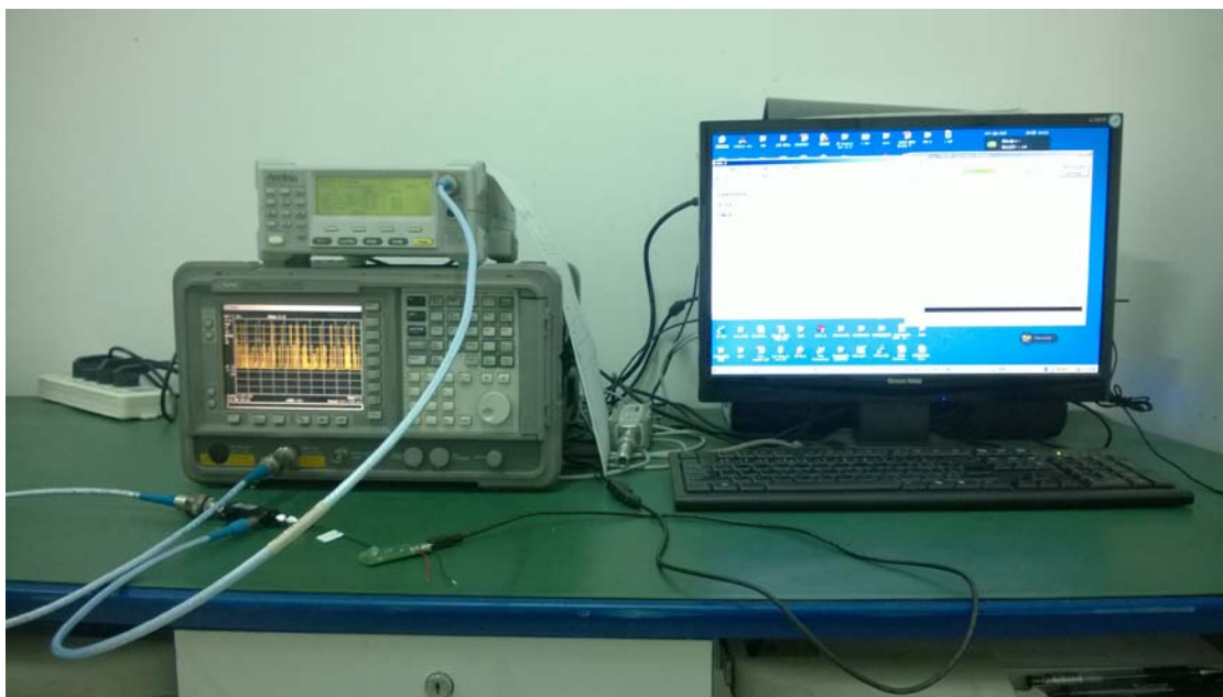
6. Conducted emission antenna's port
