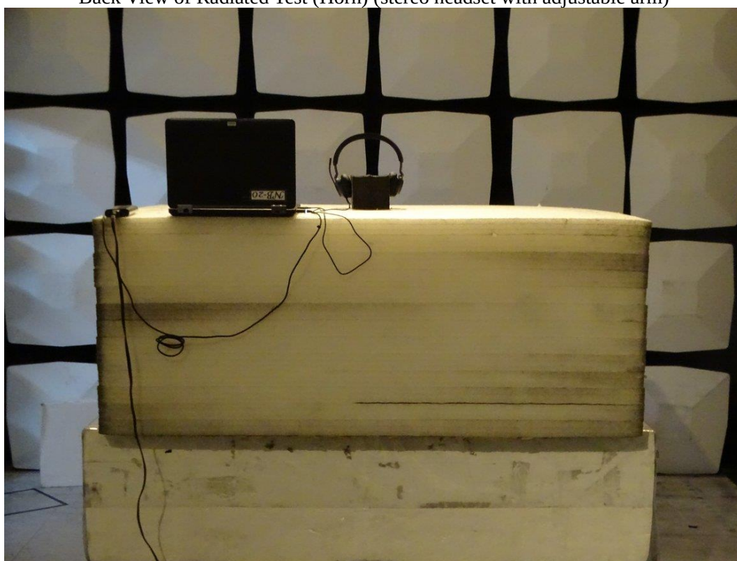
Back View of Radiated Test (Horn) (stereo headset with adjustable arm)
