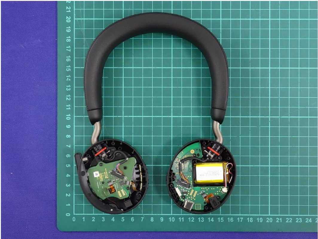
(25) EUT Photo
