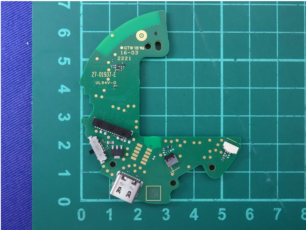
(32) EUT Photo
