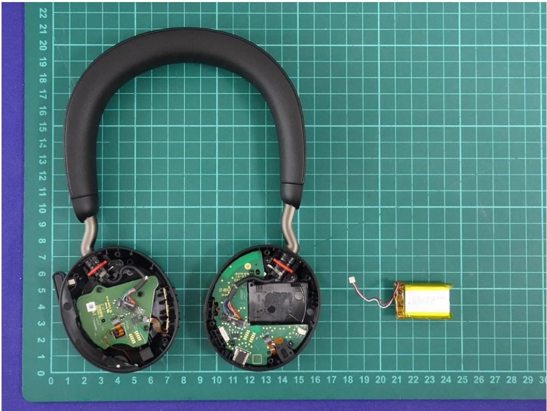
(26) EUT Photo
