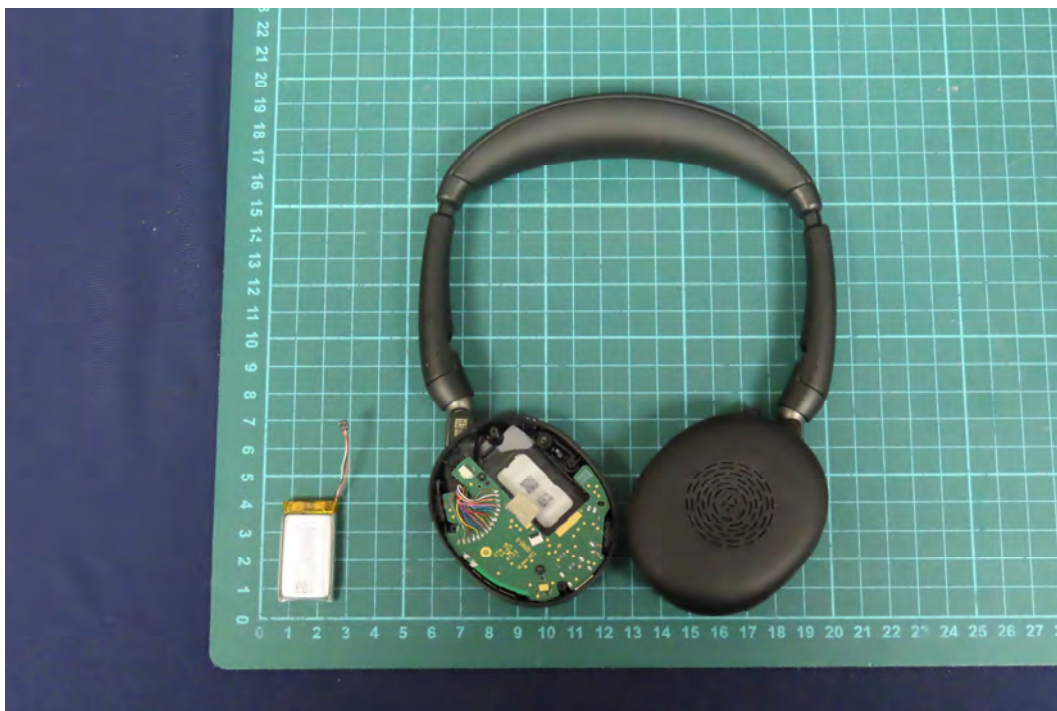
(11) EUT Photo
