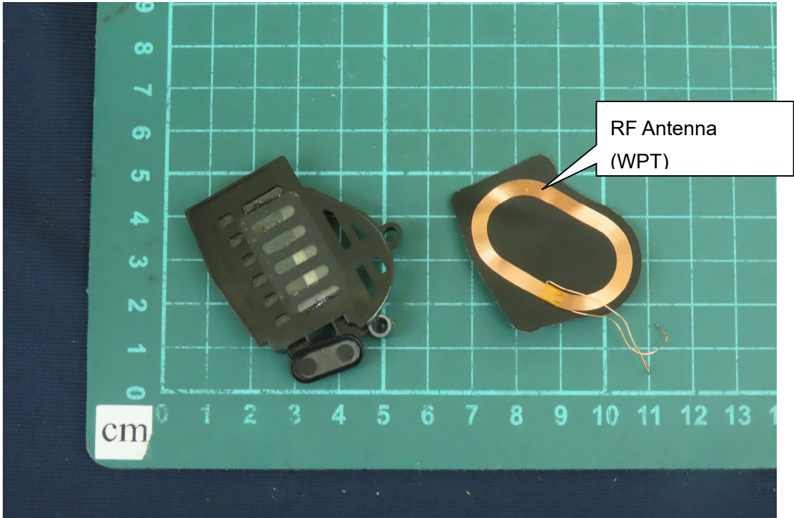
(26) EUT Photo
