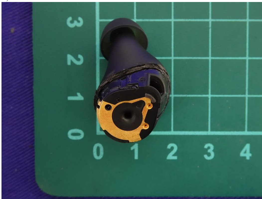
(26) EUT Photo
