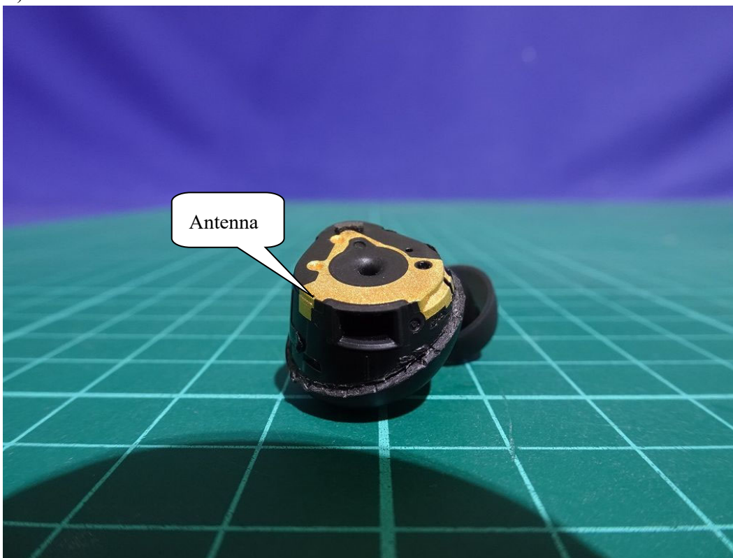
(38) EUT Photo
