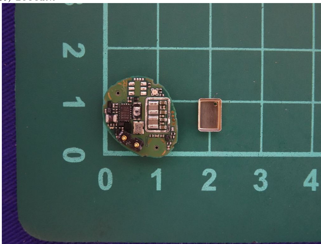
(55) EUT Photo
