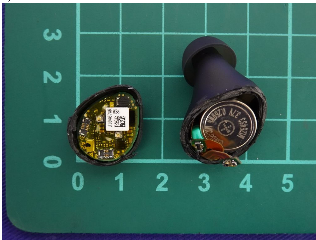
(28) EUT Photo
