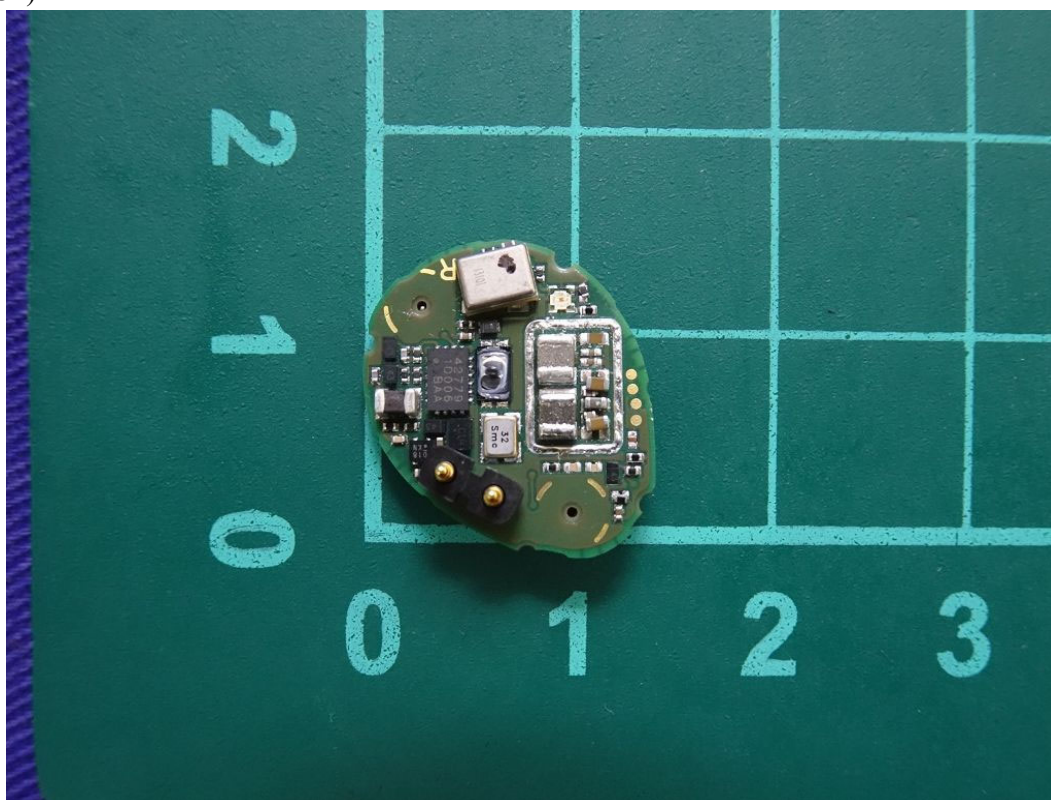
(34) EUT Photo
