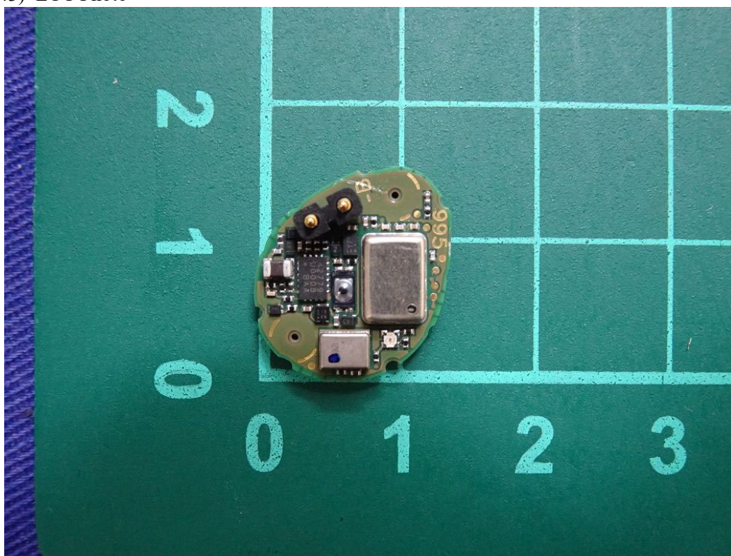
(43) EUT Photo
