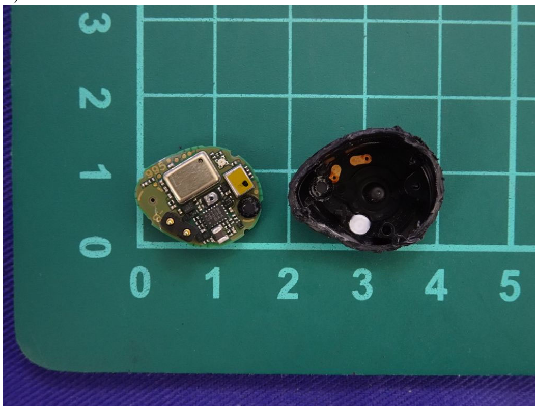
(42) EUT Photo
