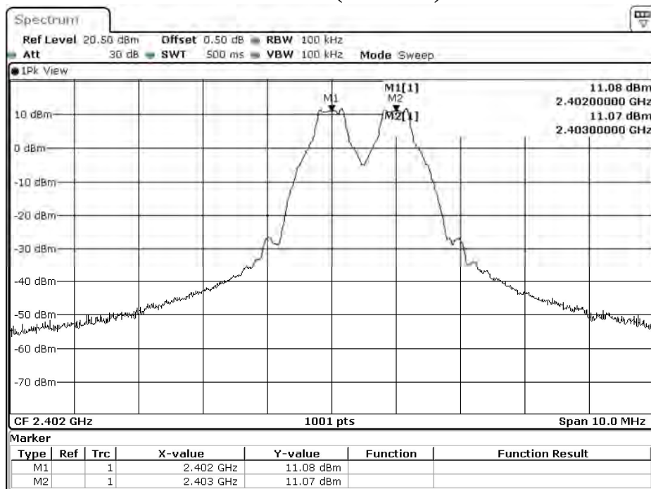
Channel 00 (2402MHz)
