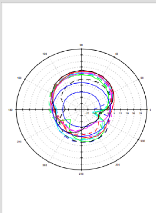
Horizontal Polarization @ CH39
