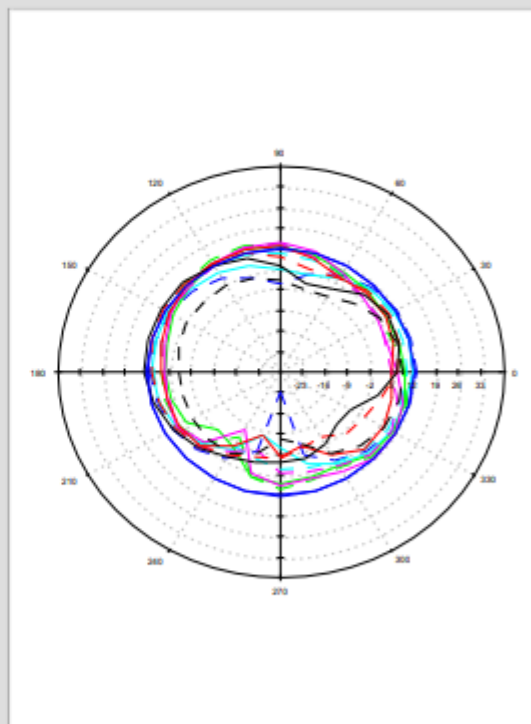
Vertical Polarization @ CH39
