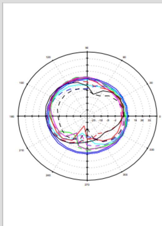
Vertical Polarization @ CH78
