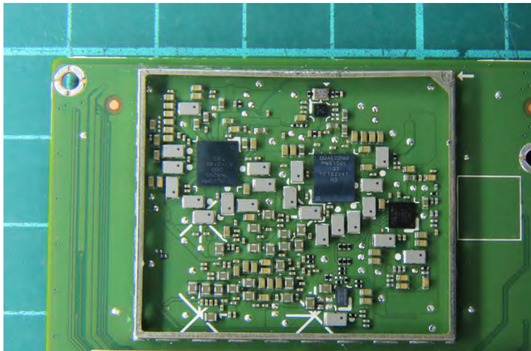
(22) EUT Photo
