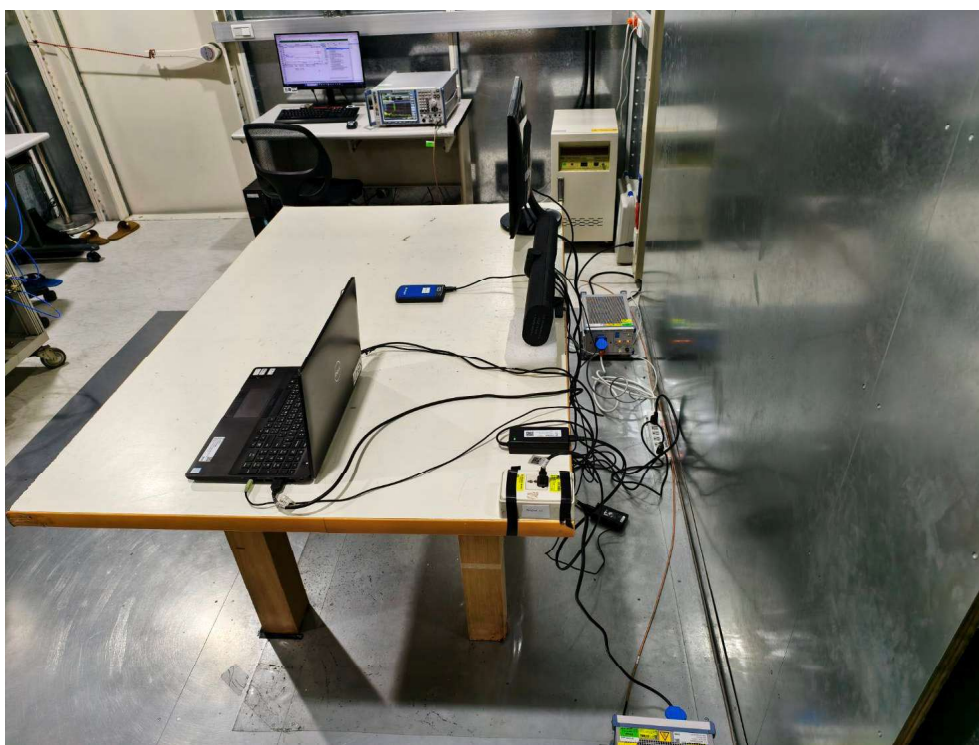
Back View of AC Power Line Conducted Emission Test
