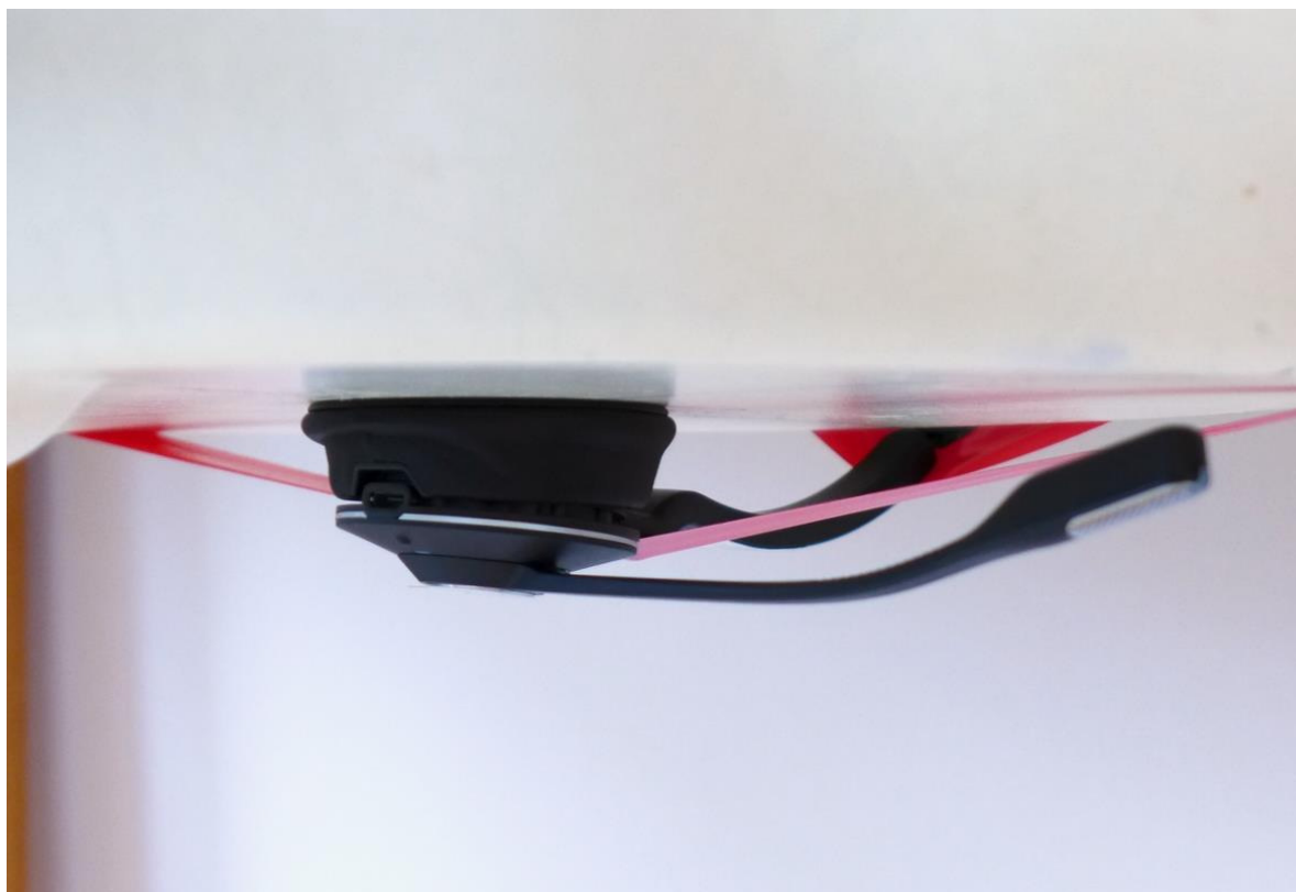
Pic. 3: Test position – inner side, 0 mm distance to phantom, antenna 1 and 2.
