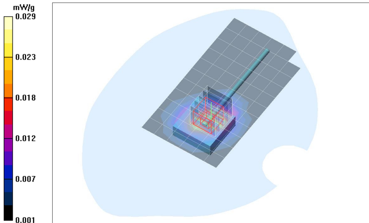
Plot. 2: SAR distribution plot for DECT, channel 4, antenna 2, flat part of the phantom.
