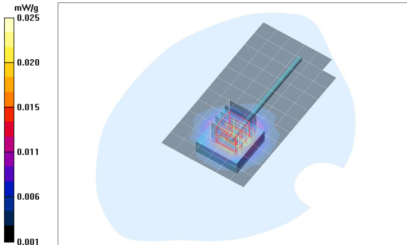
Plot. 1: SAR distribution plot for DECT, channel 4, antenna 1, flat part of the phantom.
