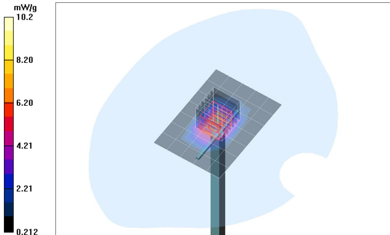
Plot. 3: System Verification Measurement 1900 MHz, Head.
