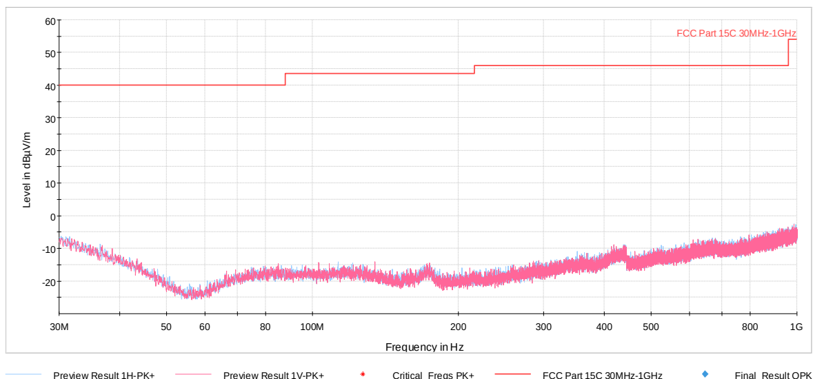
Plot 7-38. Radiated Spurious Plot below 1GHz (GFSK ePA, Pol. H & V)
