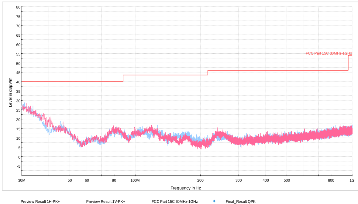
Plot 7-74. Radiated Spurious Plot below 1GHz (GFSK ePA, Pol. H & V)
