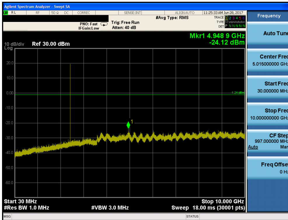
Plot 7-51. Conducted Spurious Plot (Bluetooth, GFSK, ePA – Ch. 39)
