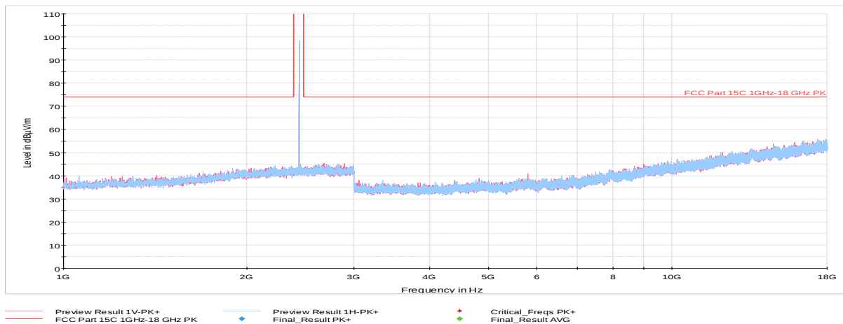
Plot 7-62. Radiated Spurious Plot above 1GHz (BT ePA – Ch. 39, Ant. Pol. H & V)
