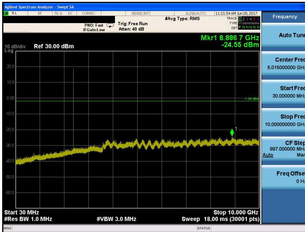
Plot 7-49. Conducted Spurious Plot (Bluetooth, GFSK, ePA – Ch. 0)
