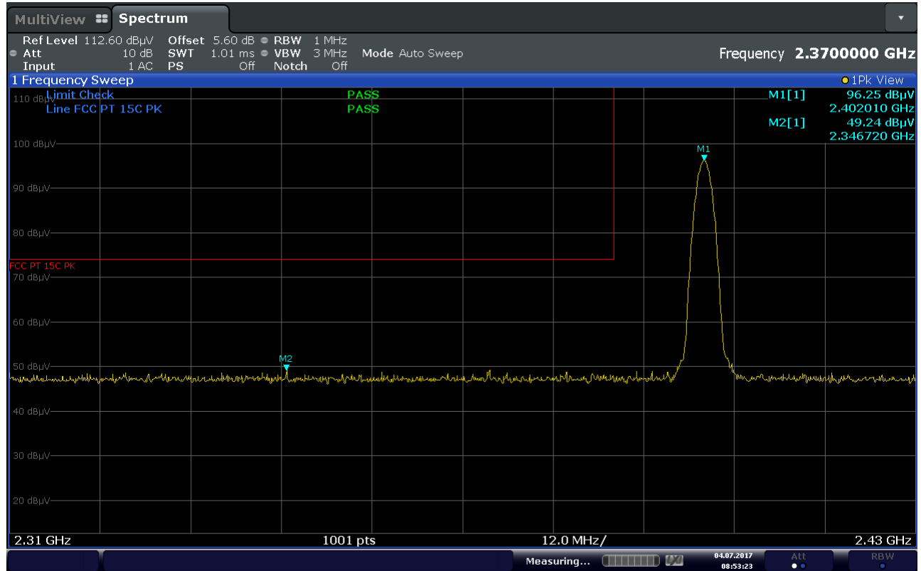
Plot 7-69. Radiated Restricted Lower Band Edge Measurement (Peak)
