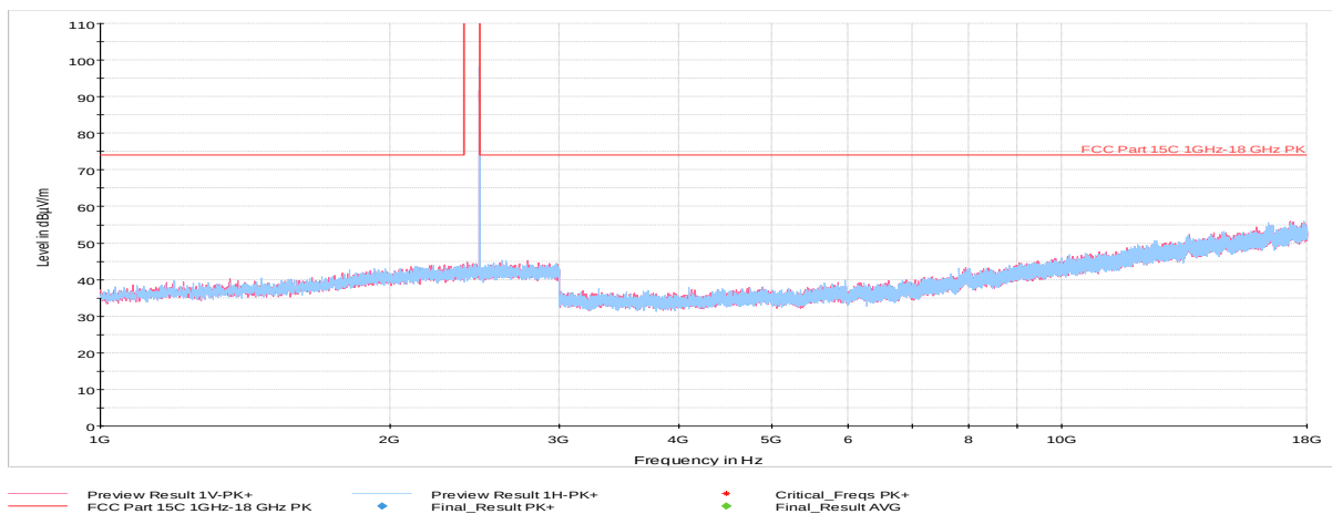
Plot 7-63. Radiated Spurious Plot above 1GHz (BT ePA – Ch. 78, Ant. Pol. H & V)
