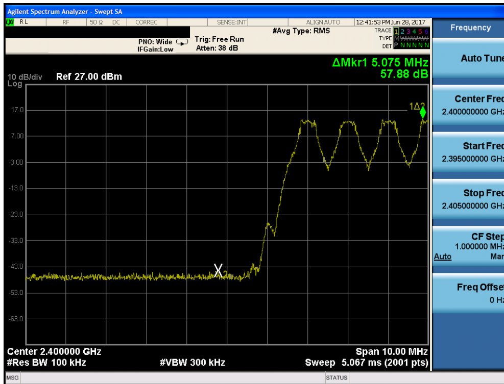
Plot 7-31. Band Edge Plot (Bluetooth with Hopping Enabled, GFSK, iPA - Ch.0)
