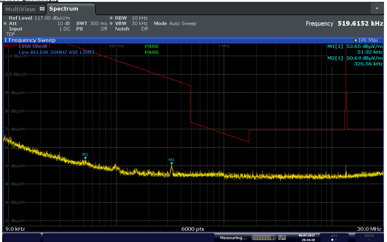
Plot 7-1. Radiated Spurious Plot 9kHz – 30MHz (CE A 848kbps, Pol. X)
