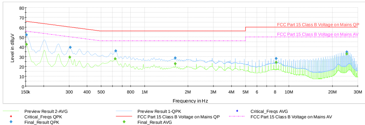
Plot 7-50. Line Conducted Plot with 802.11b (L1)
