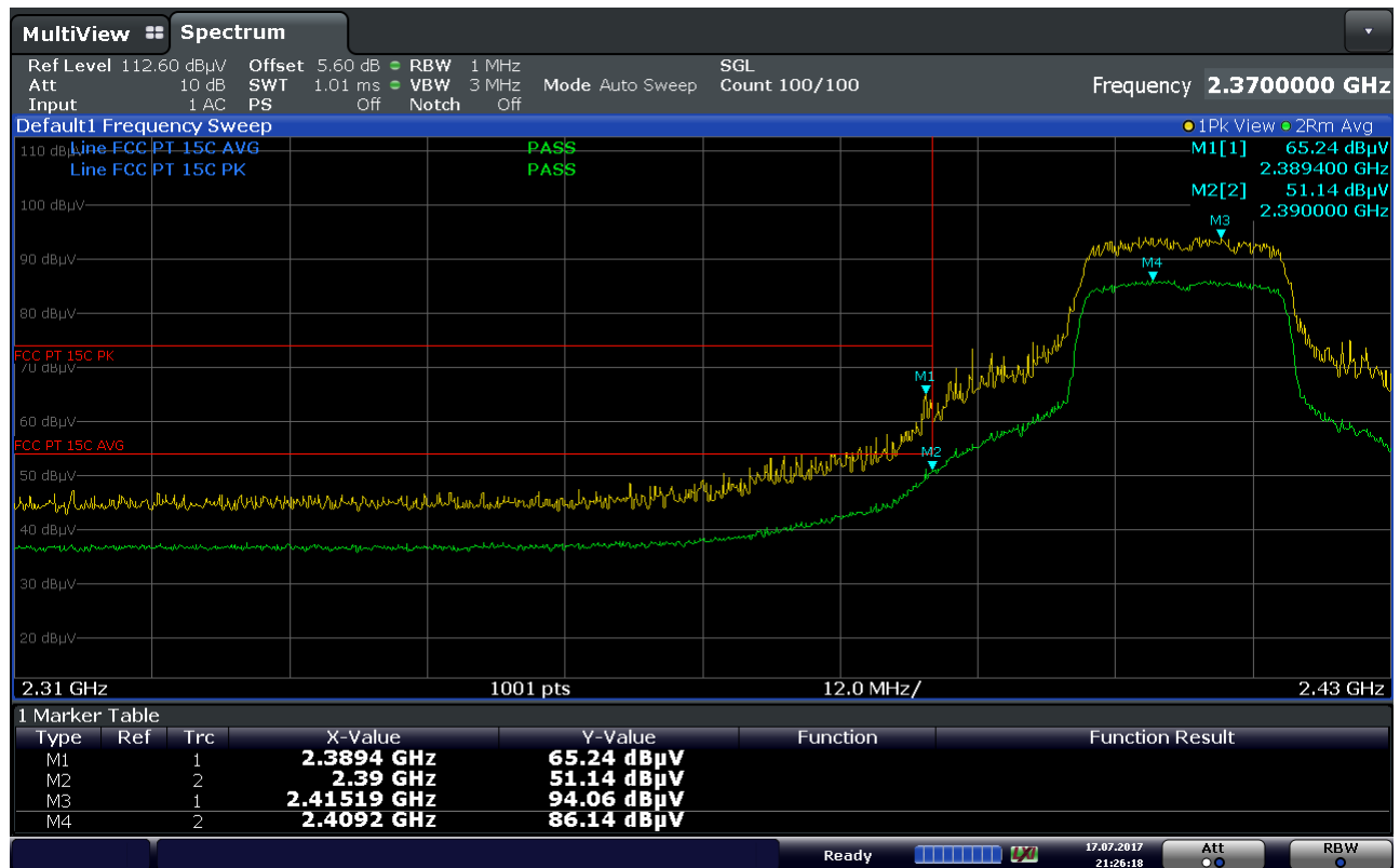
Plot 7-44. Radiated Restricted Lower Band Edge Measurement (Average & Peak)
