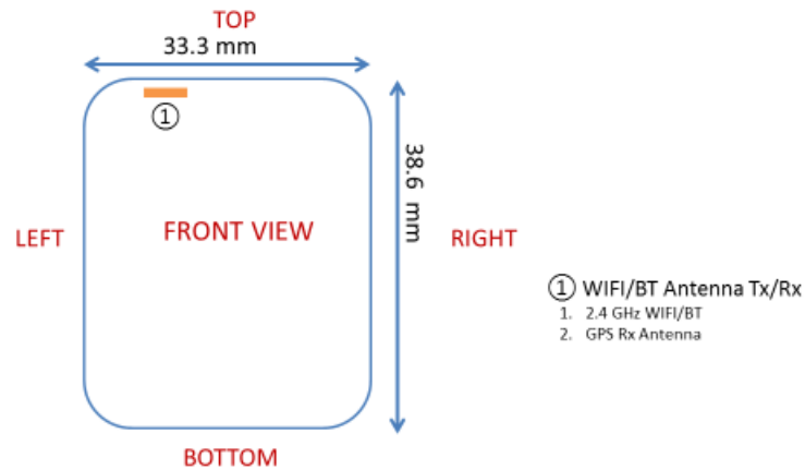
Figure F-1 DUT Antenna Locations
