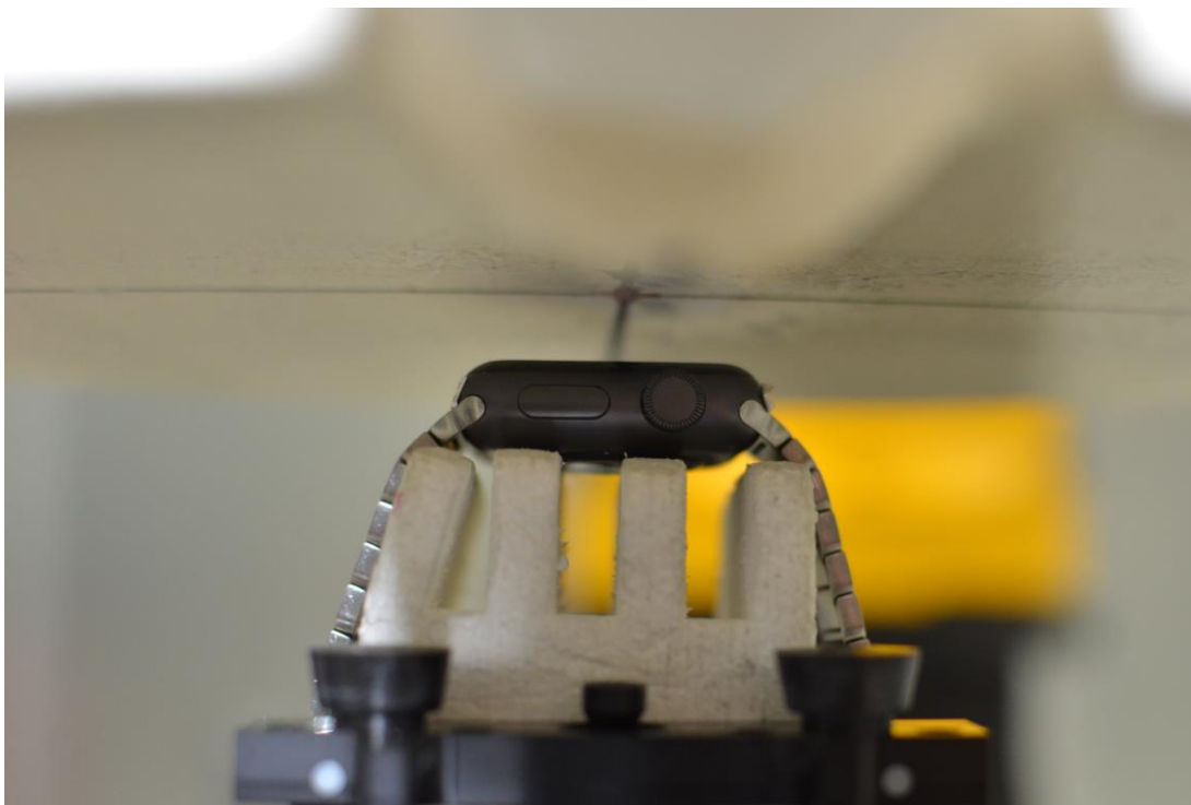
SAR Test Setup Photo 2: Aluminum front side at 1.0 cm with metal links wrist band
