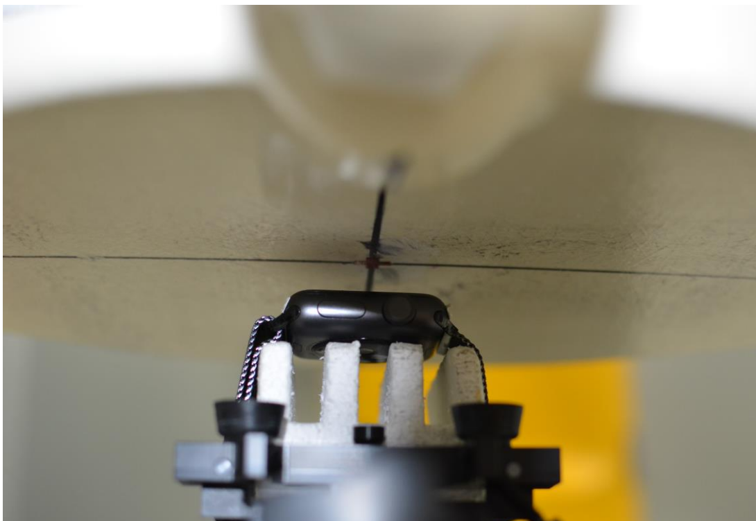
SAR Test Setup Photo 1: Aluminum front side at 1.0 cm with metal loop wrist band
