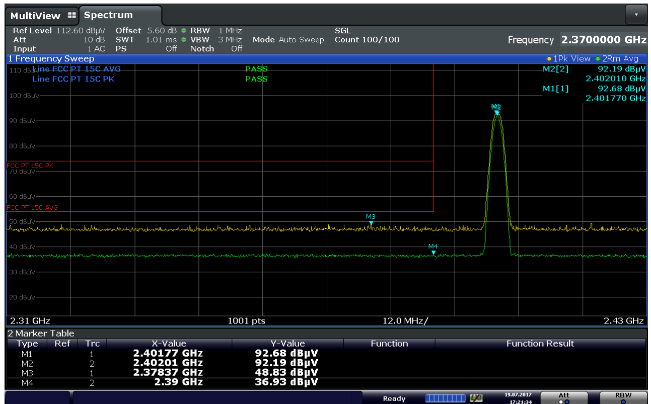
Plot 7-35. Radiated Restricted Lower Band Edge Measurement (Average & Peak)
