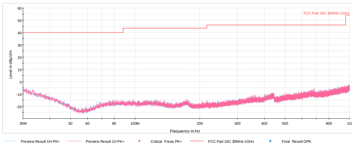
Plot 7-38. Radiated Spurious Plot below 1GHz (GFSK ePA, Pol. H & V)
