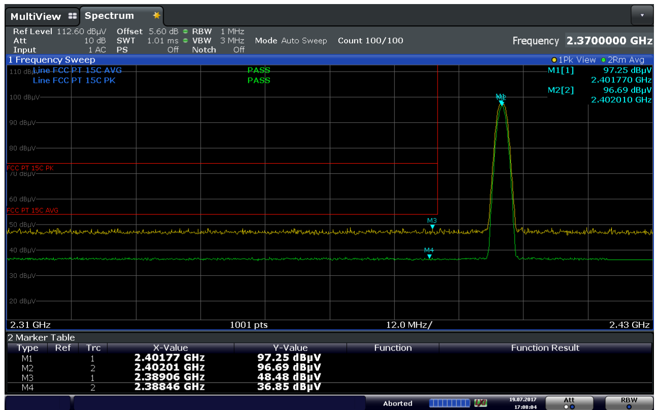
Plot 7-34. Radiated Restricted Lower Band Edge Measurement (Average & Peak)
