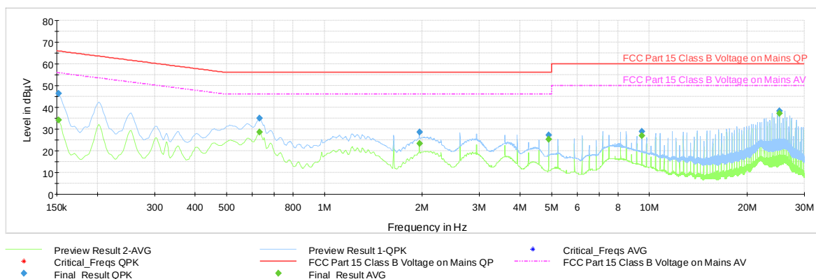
Plot 7-39. Line Conducted Plot with Bluetooth LE (GFSK ePA, L1)
