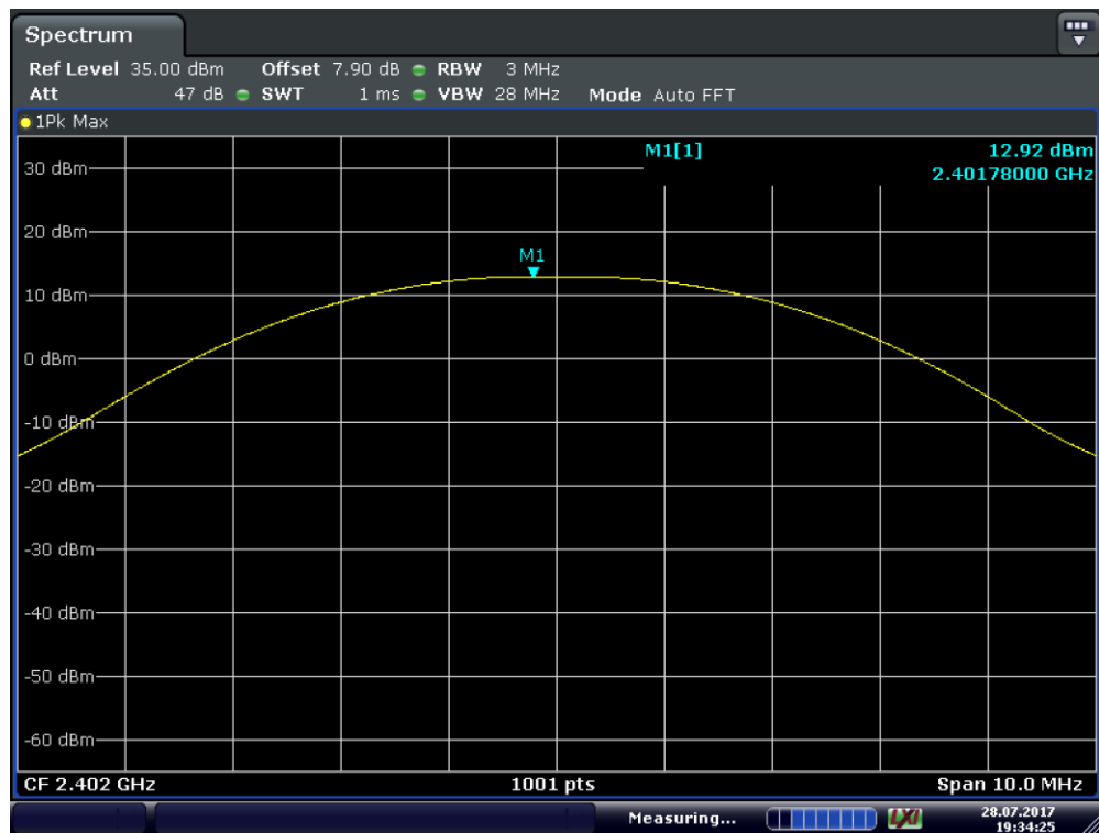
Plot 7-10. Peak Power Plot (Bluetooth (LE), iPA – Ch. 0)
