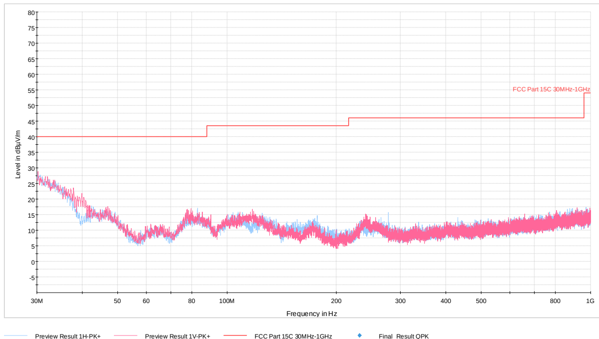
Plot 7-2. Radiated Spurious Plot 30MHz – 1GHz (CE A 848kbps, Pol. X)
