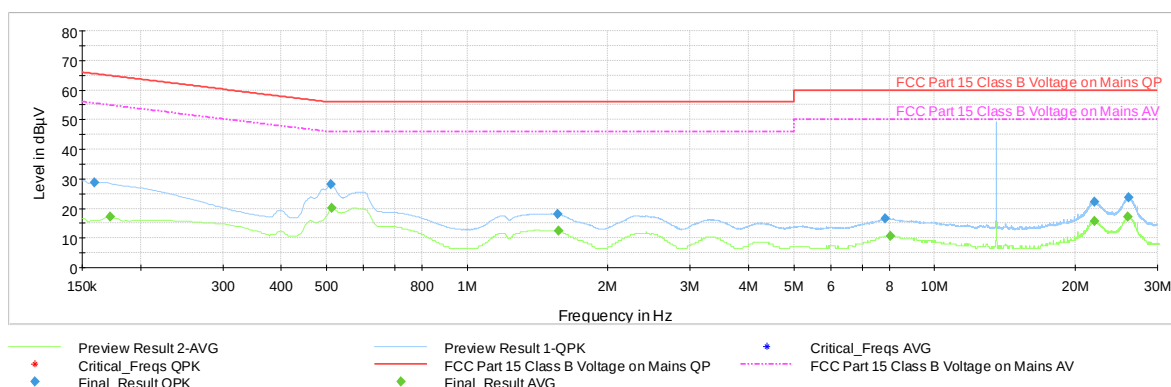
Plot 7-3. Line-Conducted Test Plot (L1)
