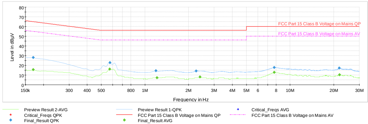
Plot 7-51. Line Conducted Plot with 802.11b (N)
