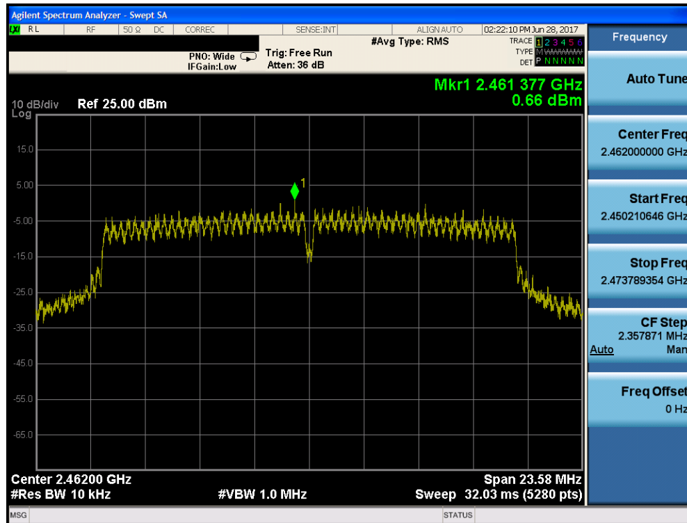
Plot 7-18. Power Spectral Density Plot (802.11n (2.4GHz) – Ch. 11)
