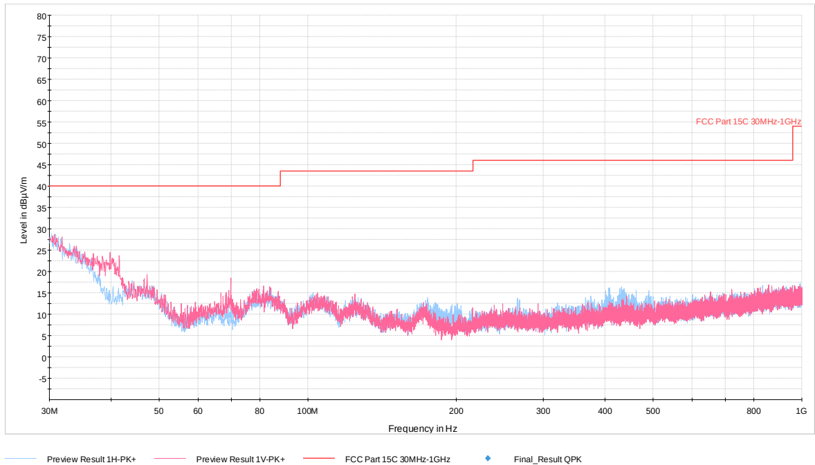
Plot 7-49. Radiated Spurious Plot below 1GHz (802.11b – Ch. 6, Pol. H & V)
