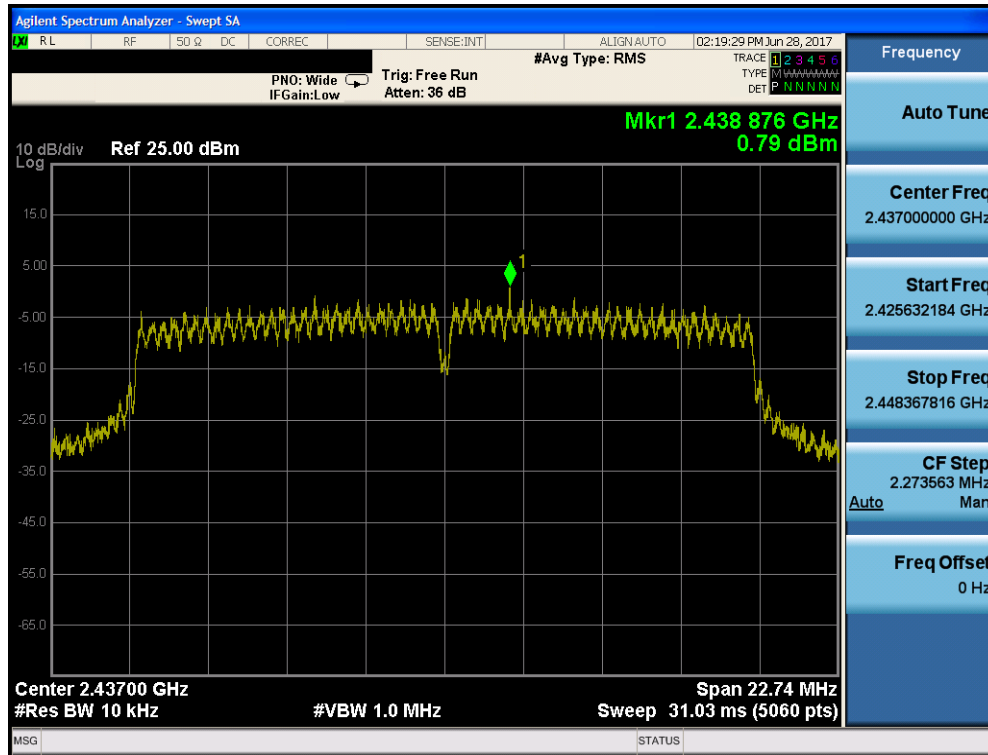
Plot 7-17. Power Spectral Density Plot (802.11n (2.4GHz) – Ch. 6)
