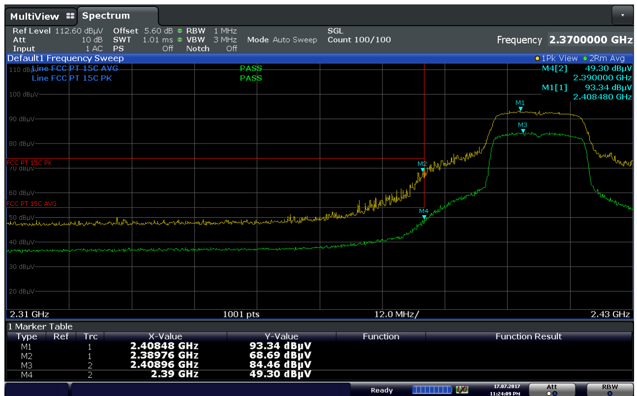
Plot 7-44. Radiated Restricted Lower Band Edge Measurement (Average & Peak)
