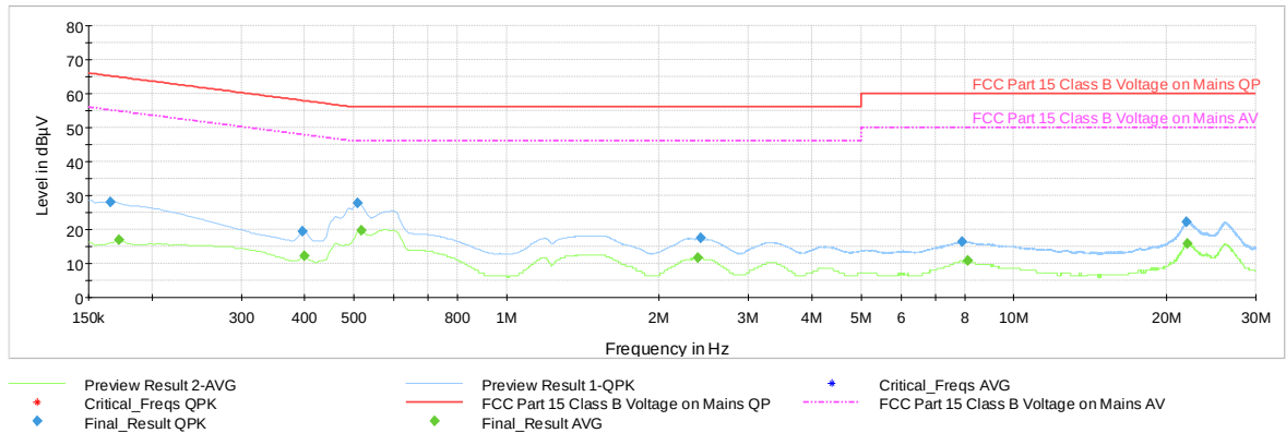
Plot 7-50. Line Conducted Plot with 802.11b (L1)
