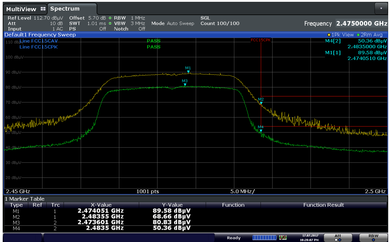
Plot 7-48. Radiated Restricted Upper Band Edge Measurement (Average & Peak)
