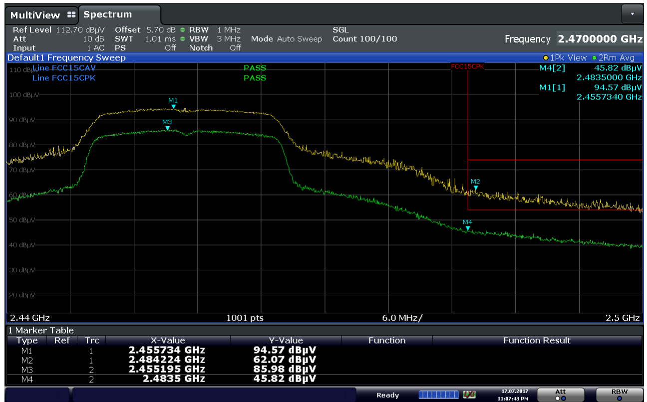
Plot 7-45. Radiated Restricted Upper Band Edge Measurement (Average & Peak)
