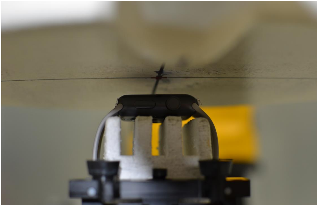
SAR Test Setup Photo 3: Aluminum front side at 1.0 cm with sport wrist band
