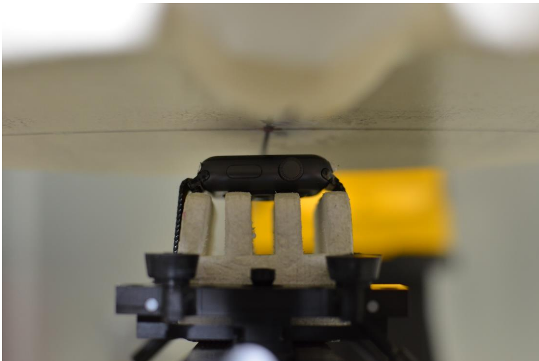
SAR Test Setup Photo 1: Aluminum front side at 1.0 cm with metal Loop wrist band
