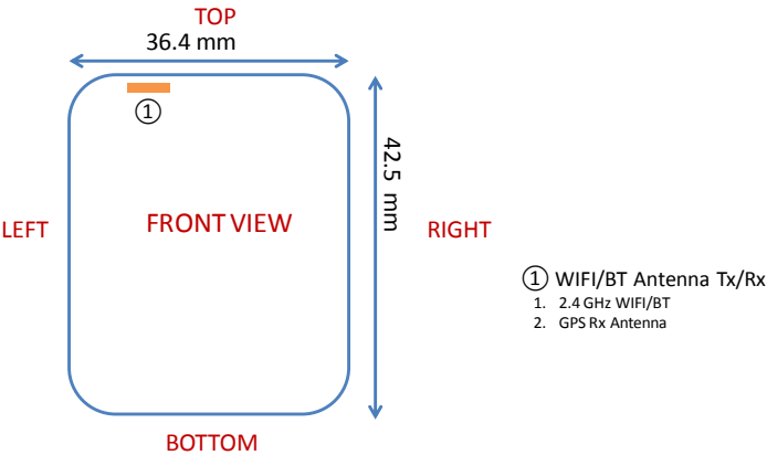
Figure F-1 DUT Antenna Locations
