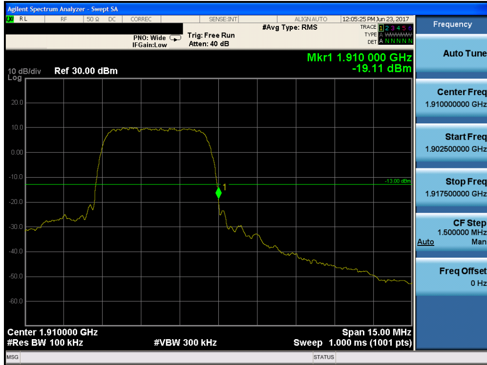
Plot 7-39. Band Edge Plot (PCS WCDMA Mode – Ch. 9538)
