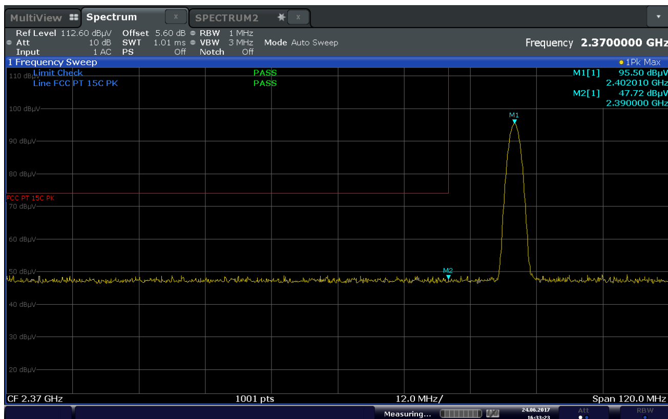
Plot 7-69. Radiated Restricted Lower Band Edge Measurement (Peak)
