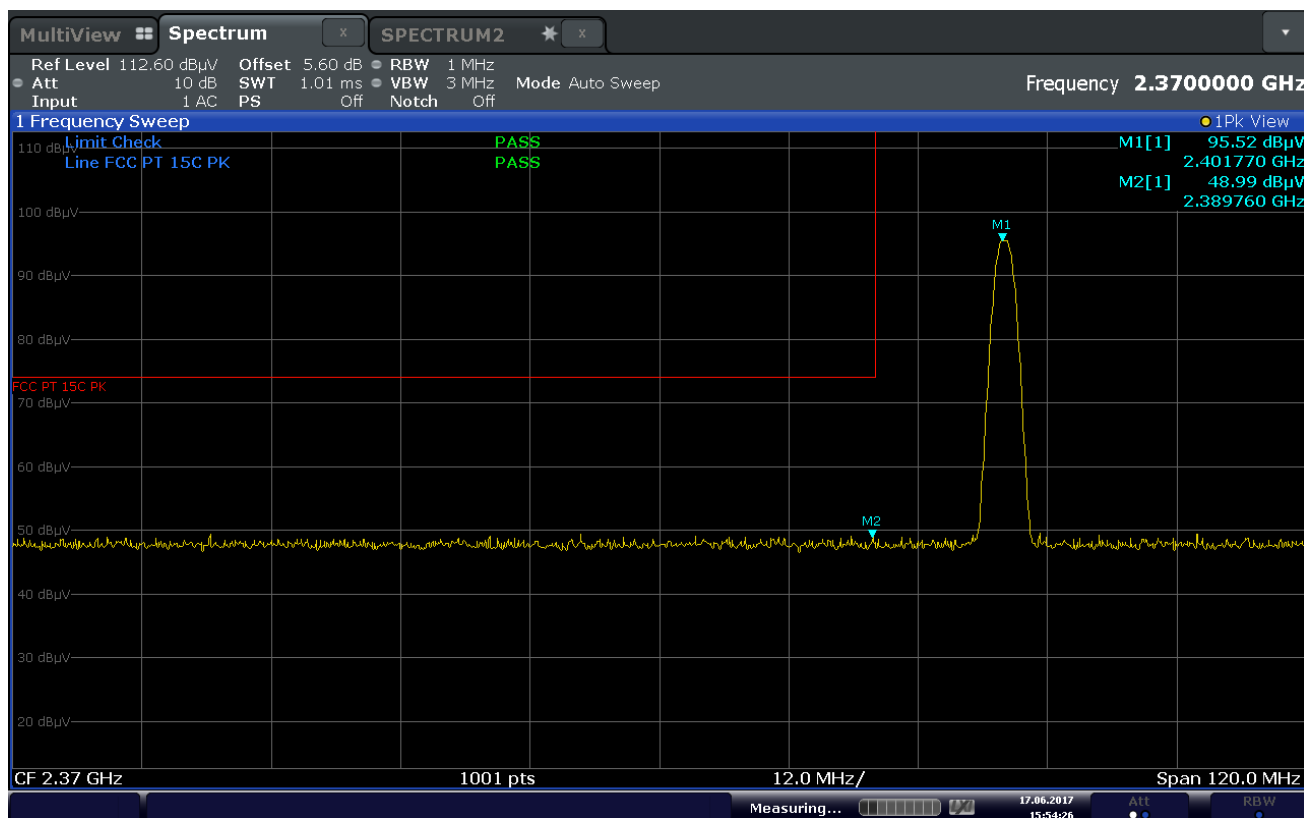
Plot 7-67. Radiated Restricted Lower Band Edge Measurement (Peak)
