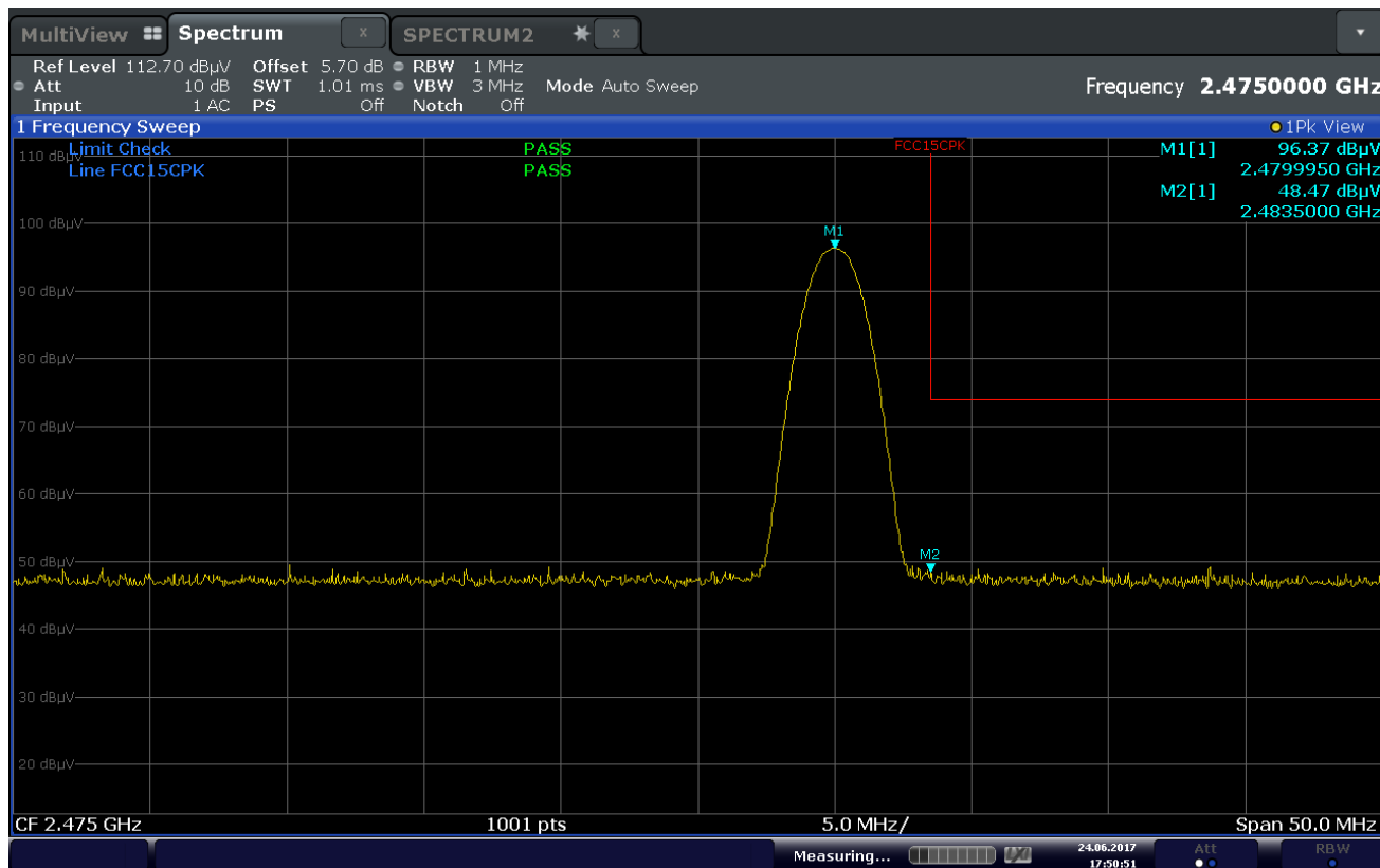
Plot 7-73. Radiated Restricted Upper Band Edge Measurement (Peak)
