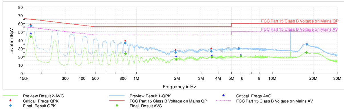
Plot 7-3. Line-Conducted Test Plot (L1)
