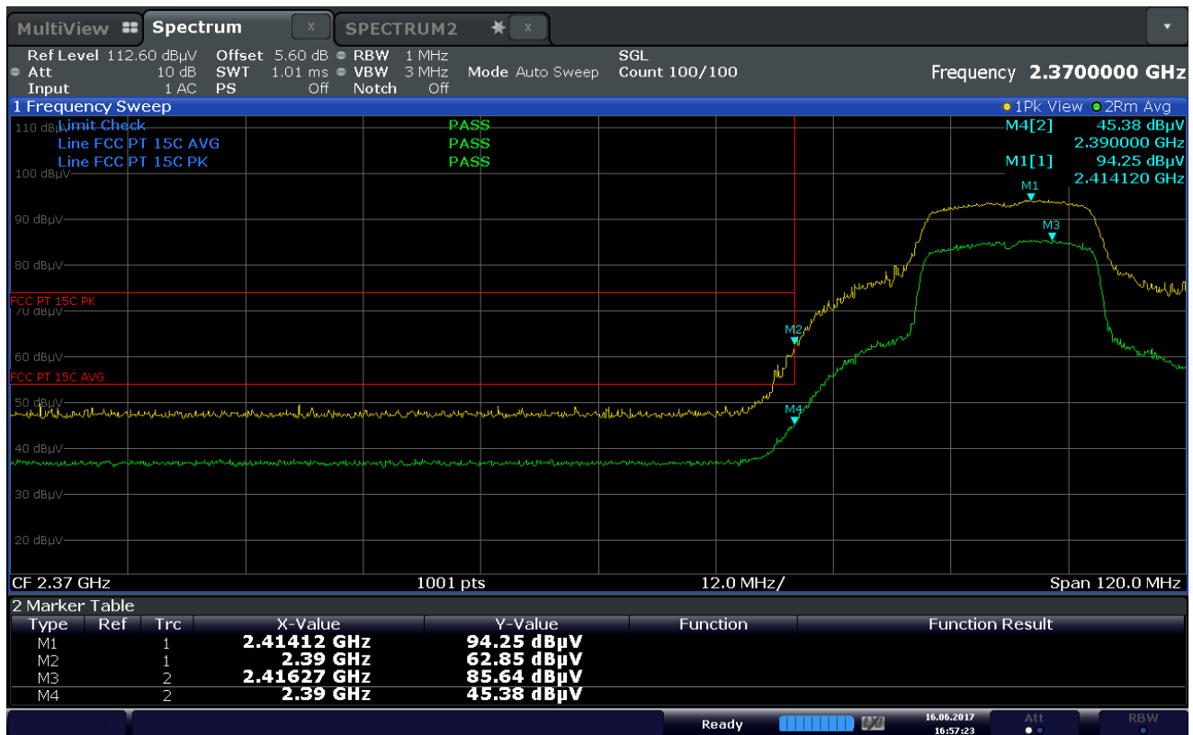
Plot 7-45. Radiated Restricted Lower Band Edge Measurement (Average & Peak)
