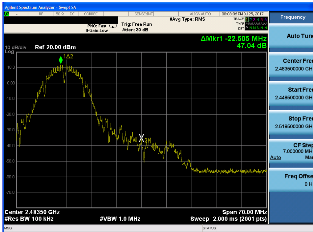
Plot 7-20. Band Edge Plot (802.11b – Ch. 11)
