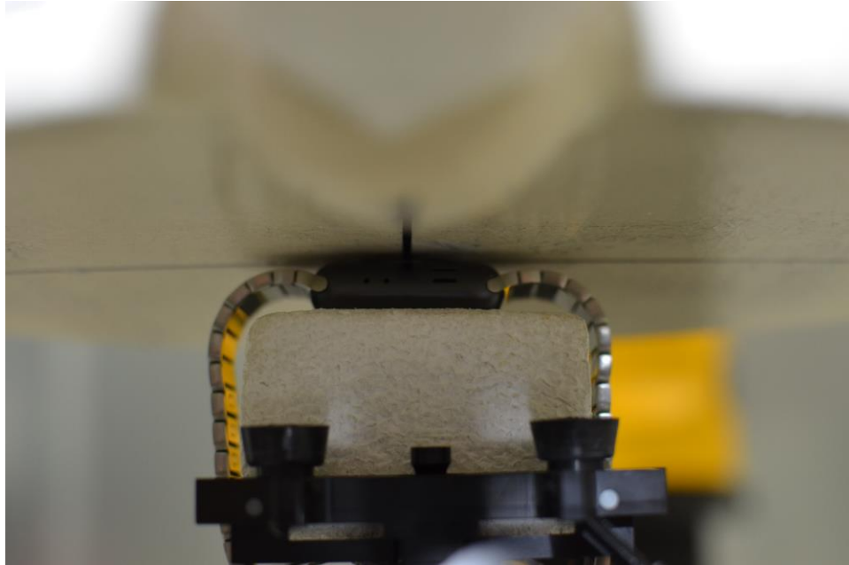
SAR Test Setup Photo 11: Aluminum with Metal Links wrist band, Back side at 0.0 cm
