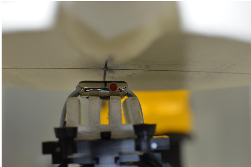
SAR Test Setup Photo 6: Stainless Steel with Sport wrist band, Front side at 1.0 cm
