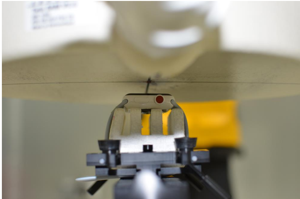
SAR Test Setup Photo 9: Ceramic with Sport wrist band, Front side at 1.0 cm
