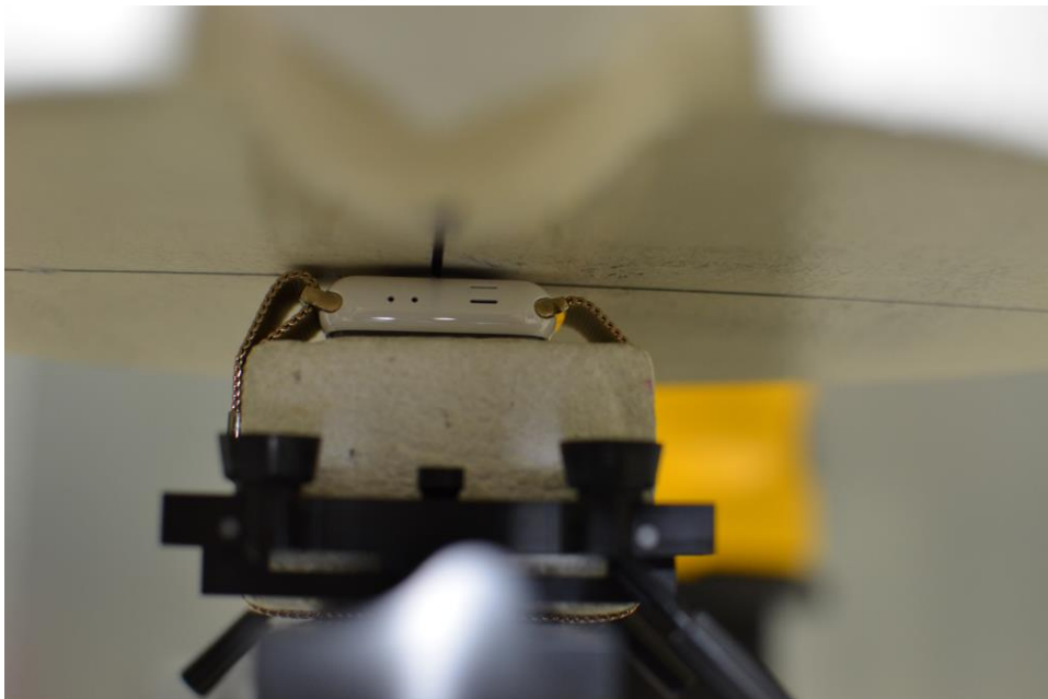
SAR Test Setup Photo 16: Ceramic with Metal Loop wrist band, Back side at 0.0 cm
