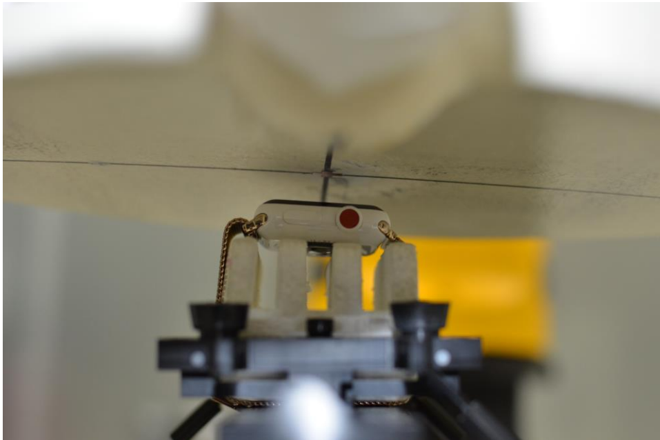
SAR Test Setup Photo 7: Ceramic with Metal Loop wrist band, Front side at 1.0 cm
