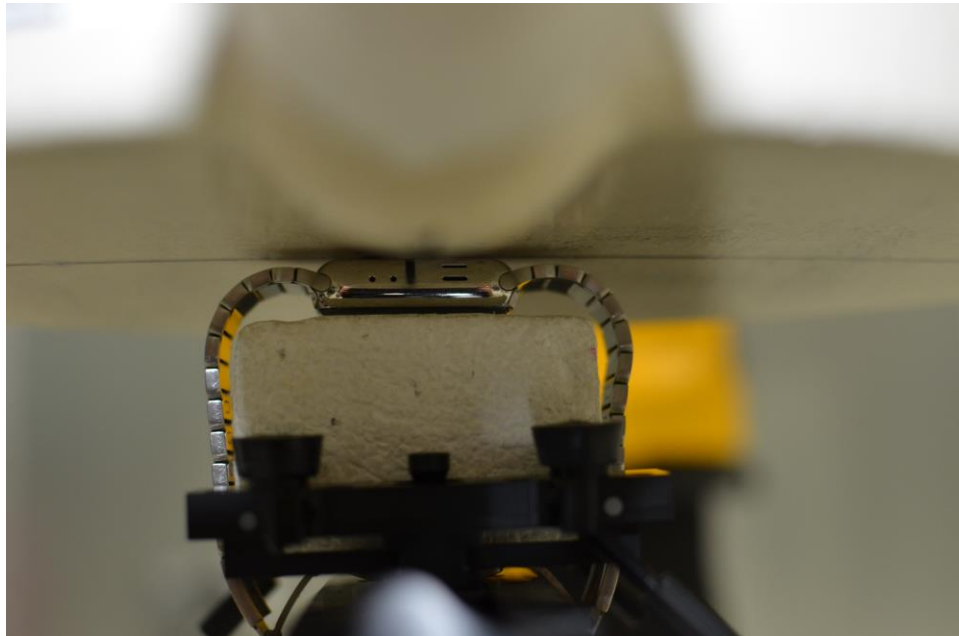
SAR Test Setup Photo 14: Stainless Steel with Metal Links wrist band, Back side at 0.0 cm
