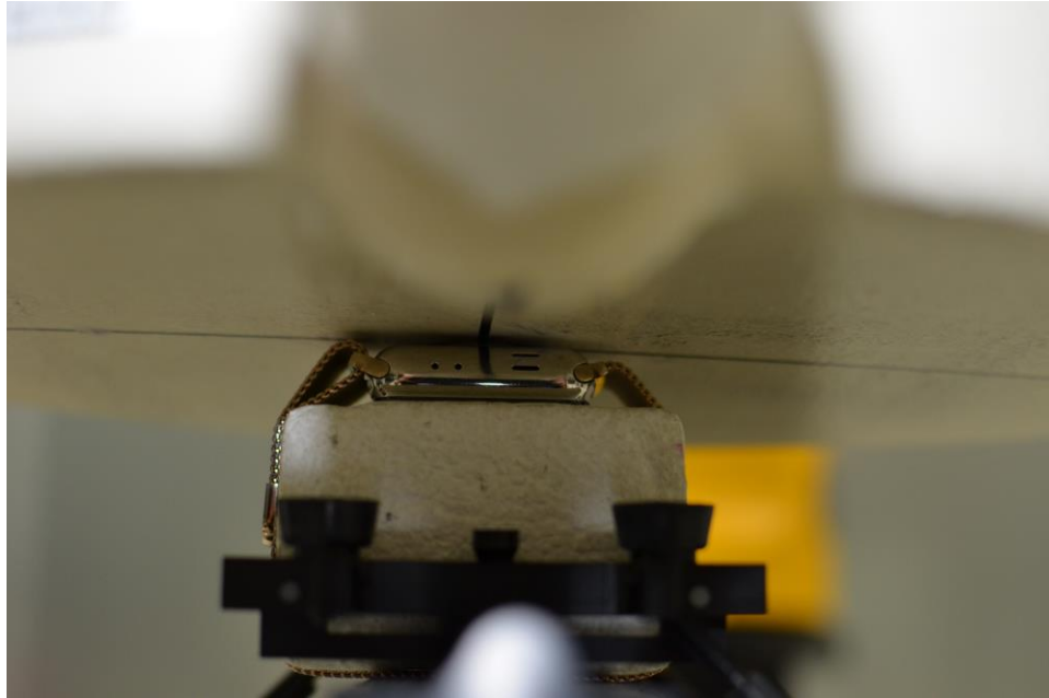
SAR Test Setup Photo 13: Stainless Steel with Metal Loop wrist band, Back side at 0.0 cm
