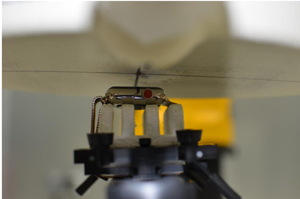
SAR Test Setup Photo 4: Stainless Steel with Metal Loop wrist band, Front side at 1.0 cm
