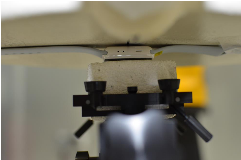
SAR Test Setup Photo 18: Ceramic with Sport wrist band, Back side at 0.0 cm
