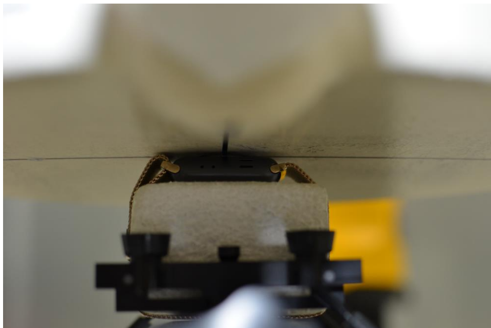
SAR Test Setup Photo 10: Aluminum with Metal Loop wrist band, Back side at 0.0 cm
