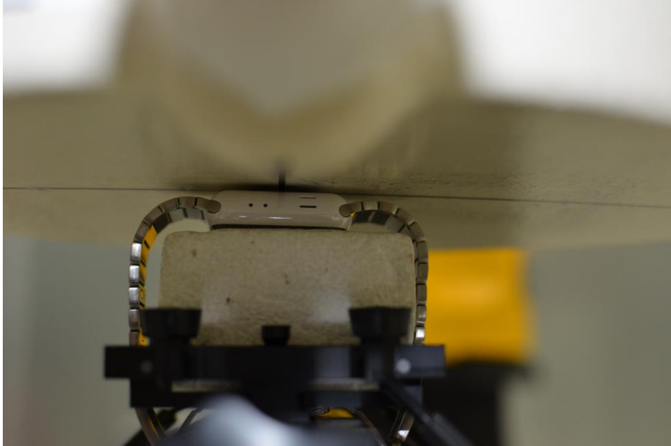
SAR Test Setup Photo 17: Ceramic with Metal Links wrist band, Back side at 0.0 cm
