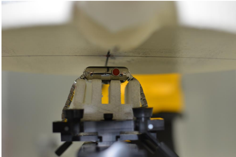
SAR Test Setup Photo 5: Stainless Steel with Metal Links wrist band, Front side at 1.0 cm
