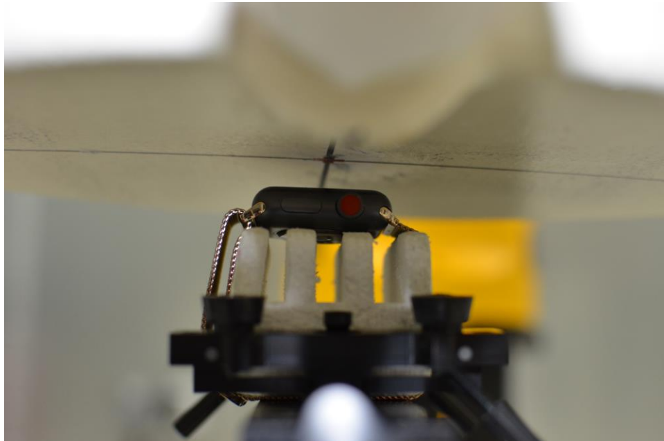
SAR Test Setup Photo 1: Aluminum with Metal Loop wrist band, Front side at 1.0 cm
