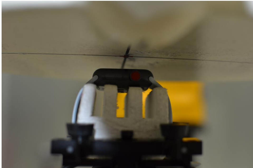
SAR Test Setup Photo 3: Aluminum with Sport wrist band, Front side at 1.0 cm
