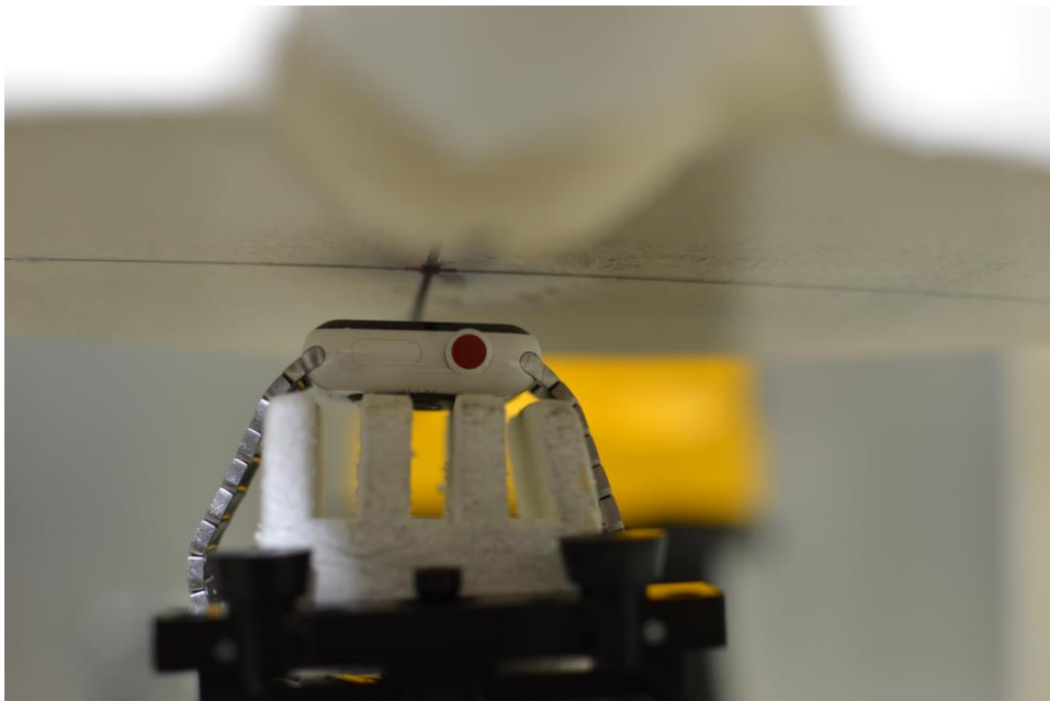
SAR Test Setup Photo 8: Ceramic with Metal Links wrist band, Front side at 1.0 cm
