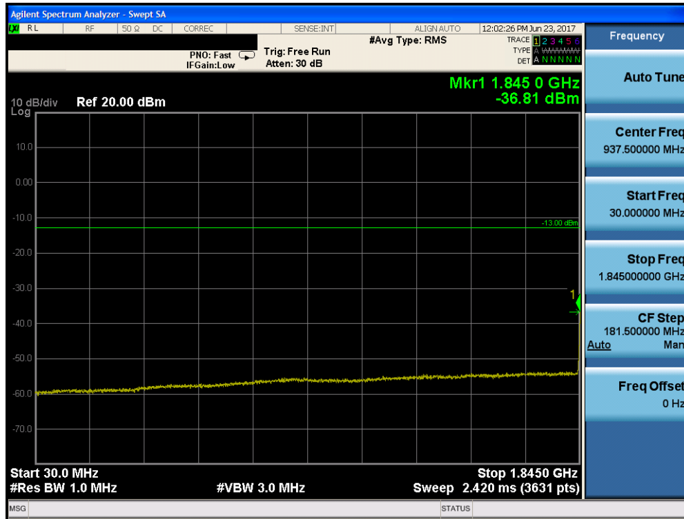
Plot 7-22. Conducted Spurious Plot (PCS WCDMA Mode – Ch. 9262)
