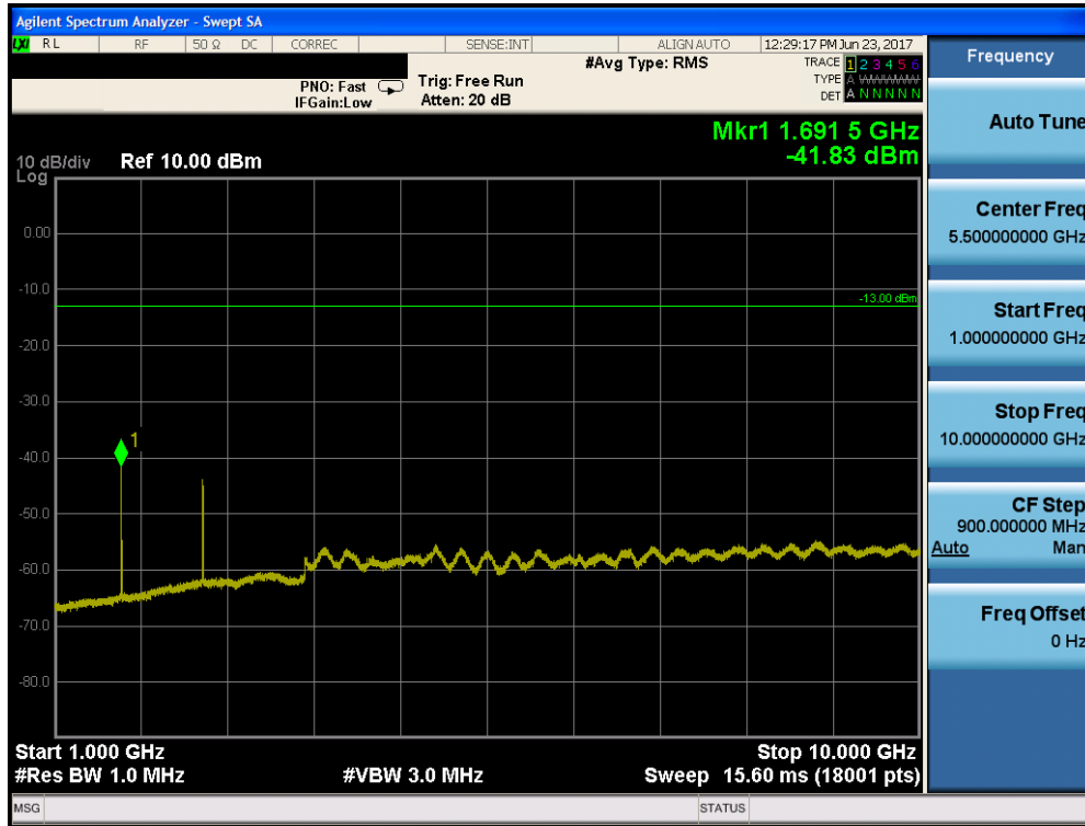
Plot 7-12. Conducted Spurious Plot (Cellular WCDMA Mode – Ch. 4233)
