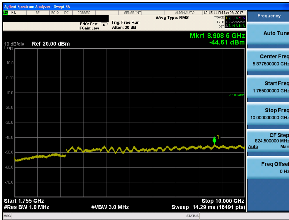
Plot 7-17. Conducted Spurious Plot (AWS WCDMA Mode – Ch. 1413)
