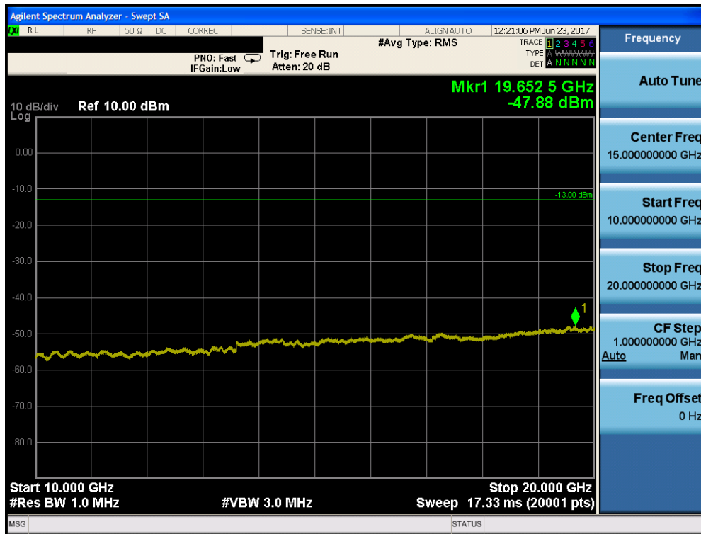
Plot 7-21. Conducted Spurious Plot (AWS WCDMA Mode – Ch. 1513)
