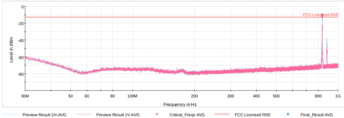
Plot 7-44. Radiated Spurious Plot (Cellular WCDMA Mode – Ch. 4183)
