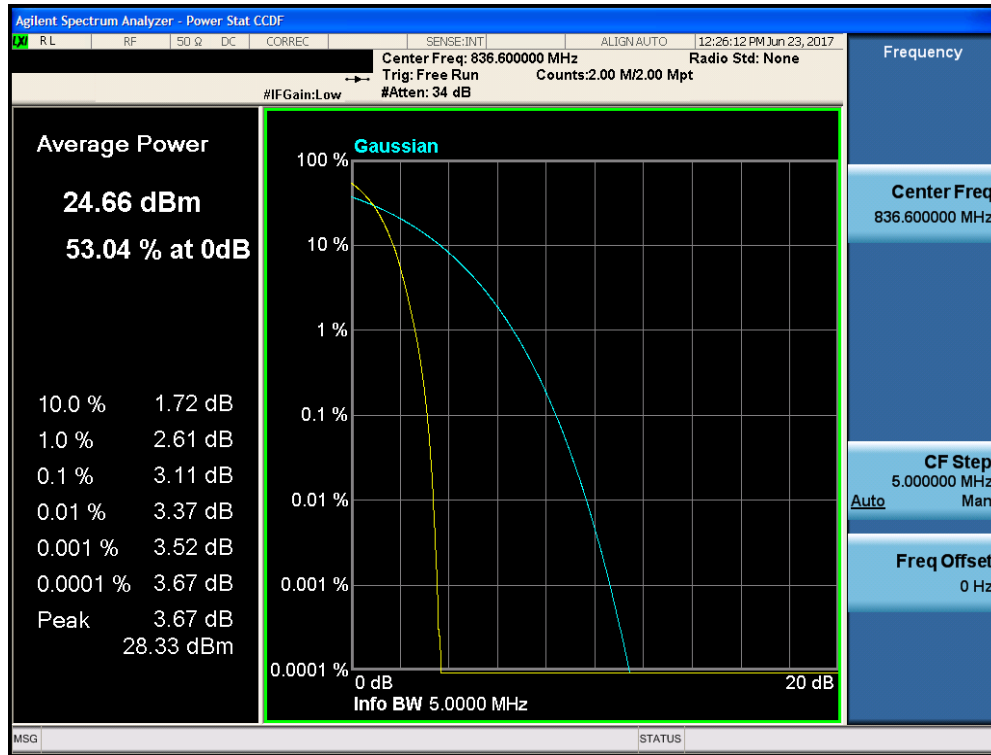
Plot 7-41. Peak-Average Ratio Plot (Cell WCDMA Mode – Ch. 4183)
