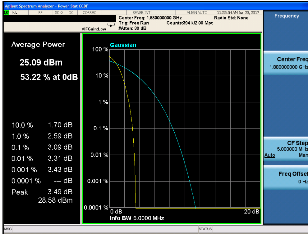
Plot 7-43. Peak-Average Ratio Plot (PCS WCDMA Mode – Ch. 9400)
