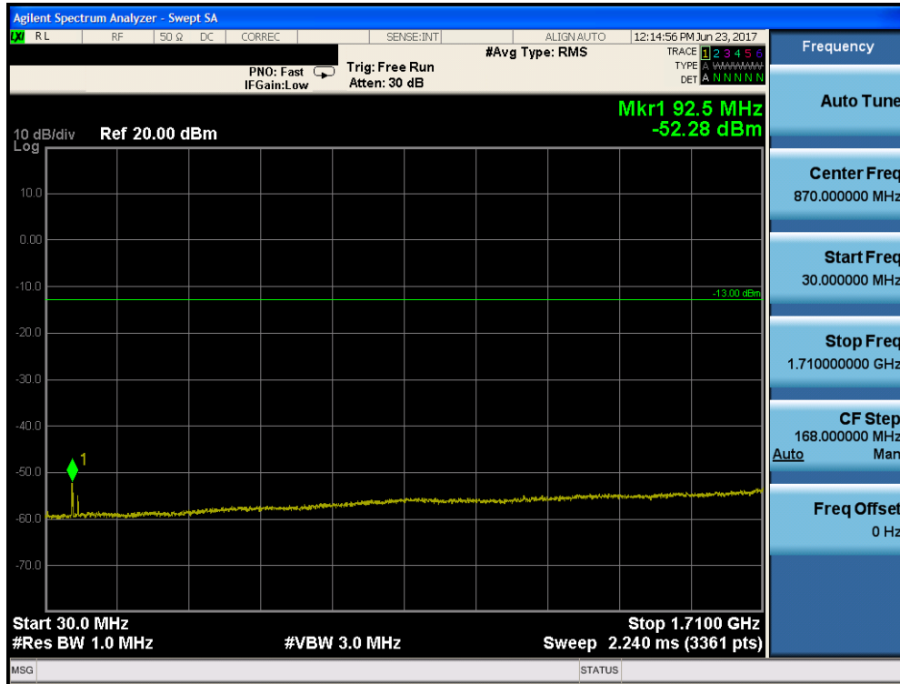
Plot 7-16. Conducted Spurious Plot (AWS WCDMA Mode – Ch. 1413)
