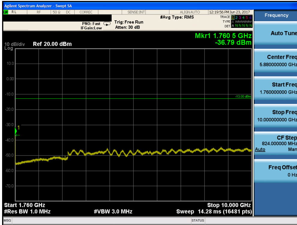
Plot 7-20. Conducted Spurious Plot (AWS WCDMA Mode – Ch. 1513)
