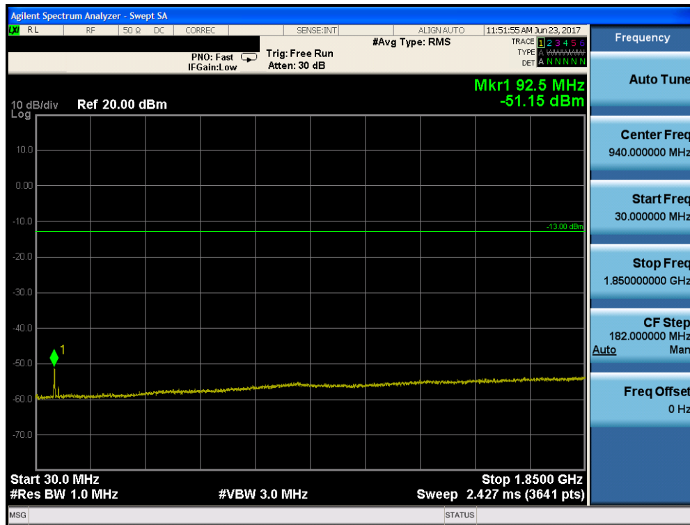
Plot 7-25. Conducted Spurious Plot (PCS WCDMA Mode – Ch. 9400)
