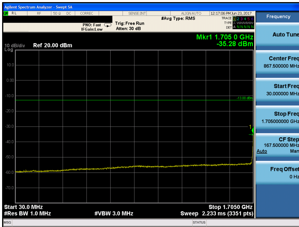
Plot 7-13. Conducted Spurious Plot (AWS WCDMA Mode – Ch. 1312)
