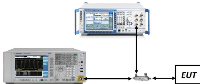
Figure 7-2. Test Instrument & Measurement Setup
