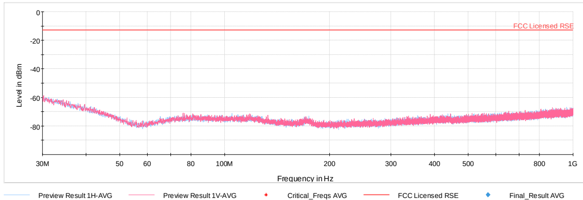
Plot 7-45. Radiated Spurious Plot (AWS WCDMA Mode – Ch. 1412)
