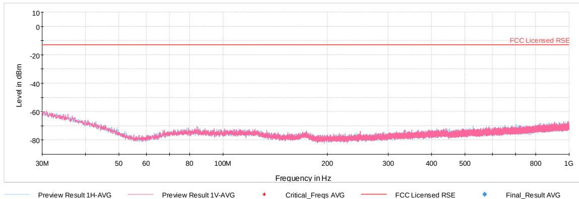
Plot 7-46. Radiated Spurious Plot (PCS WCDMA Mode – Ch. 9400)
