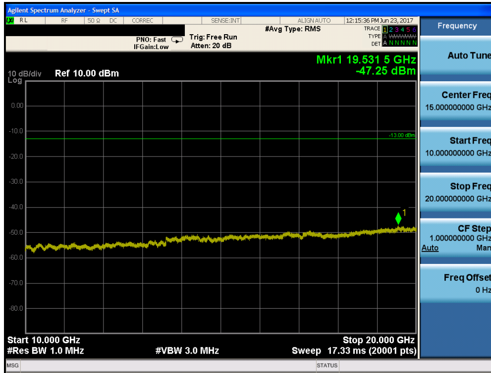
Plot 7-18. Conducted Spurious Plot (AWS WCDMA Mode – Ch. 1413)
