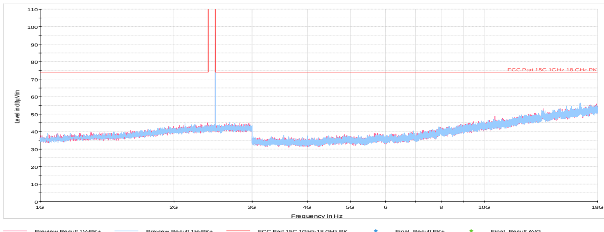
Plot 7-31. Radiated Spurious Plot above 1GHz (GFSK ePA – Ch. 78, Ant. Pol. H & V)
