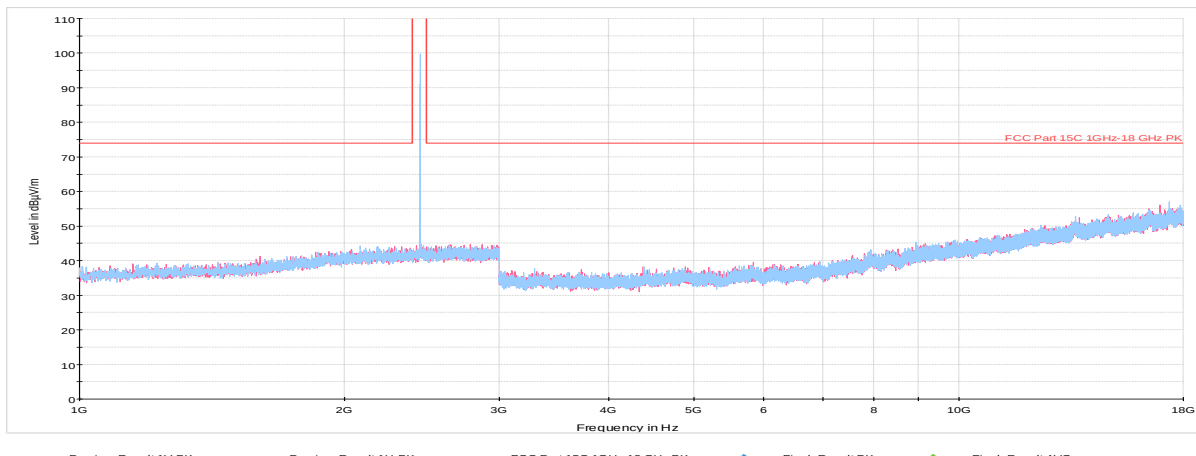
Plot 7-30. Radiated Spurious Plot above 1GHz (GFSK ePA – Ch. 39, Ant. Pol. H & V)
