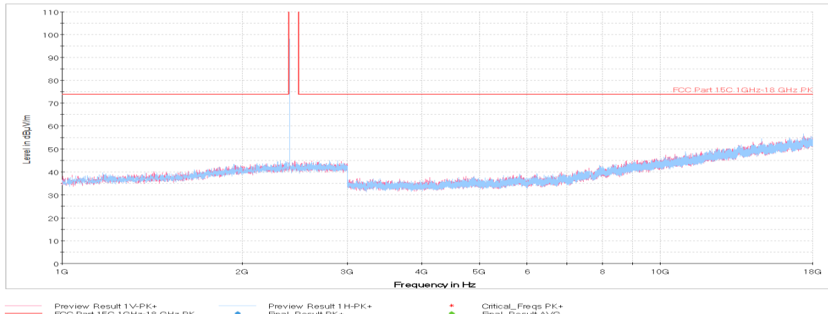
Plot 7-61. Radiated Spurious Plot above 1GHz (BT ePA- Ch. 0, Ant. Pol. H & V)
