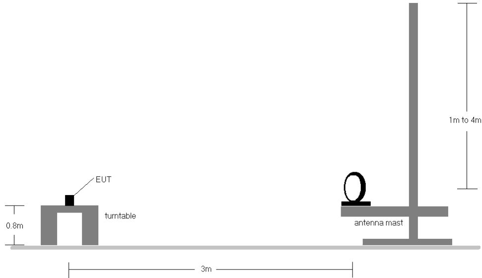
Figure 7-12. Radiated Test Setup
