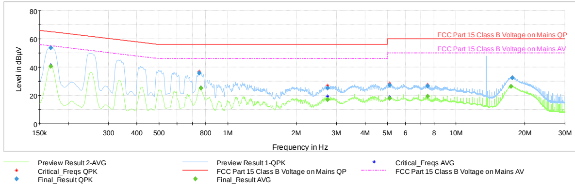
Plot 7-4. Line-Conducted Test Plot (N)
