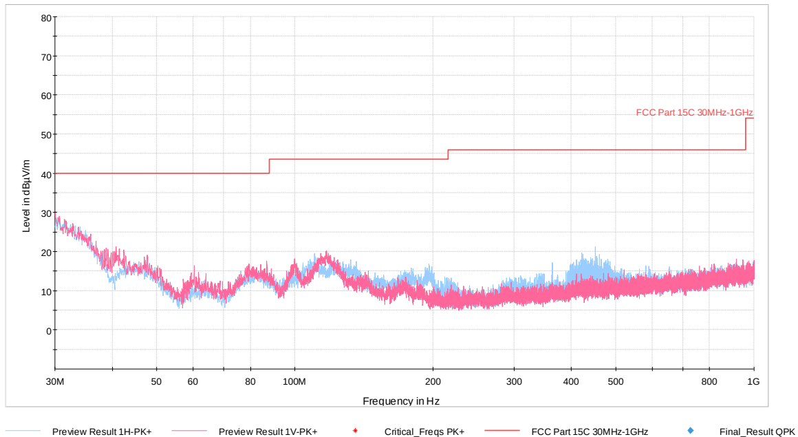
Plot 7-2. Radiated Spurious Plot 30MHz – 1GHz (CE A 484kbps, Pol. X)
