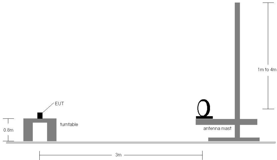
Figure 7-13. Radiated Test Setup < 30MHz
