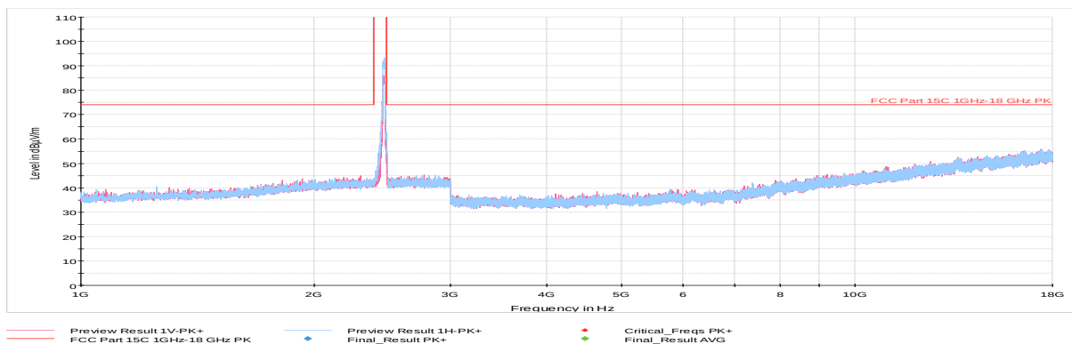
Plot 7-39. Radiated Spurious Plot above 1GHz (802.11b – Ch. 11, Ant. Pol. H & V)
