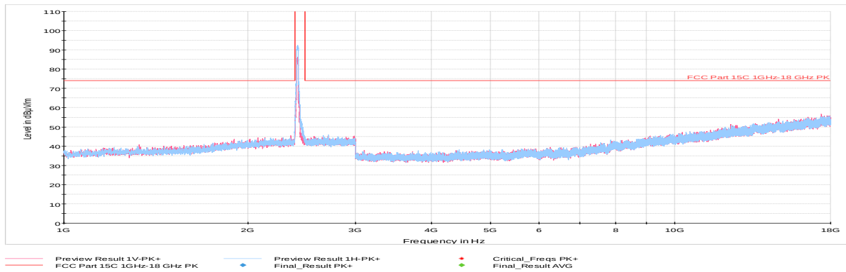
Plot 7-37. Radiated Spurious Plot above 1GHz (802.11b – Ch. 1, Ant. Pol. H & V)
