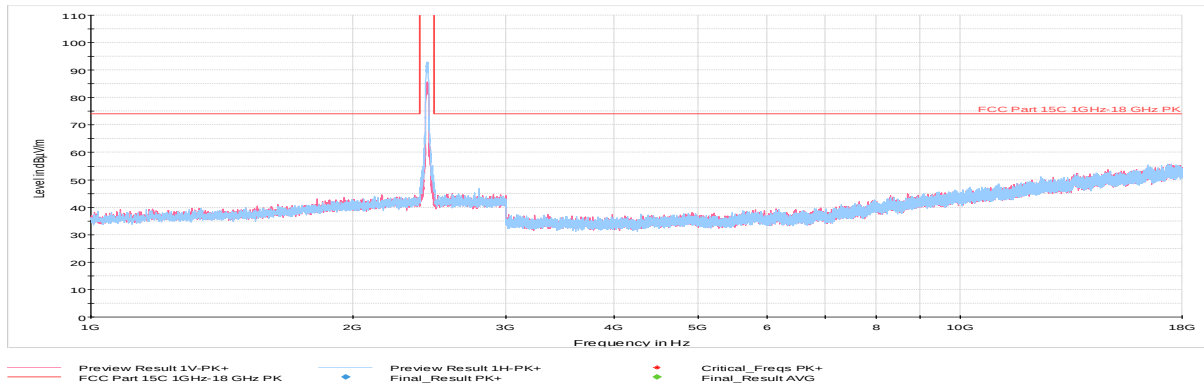
Plot 7-38. Radiated Spurious Plot above 1GHz (802.11b – Ch. 6, Ant. Pol. H & V)
