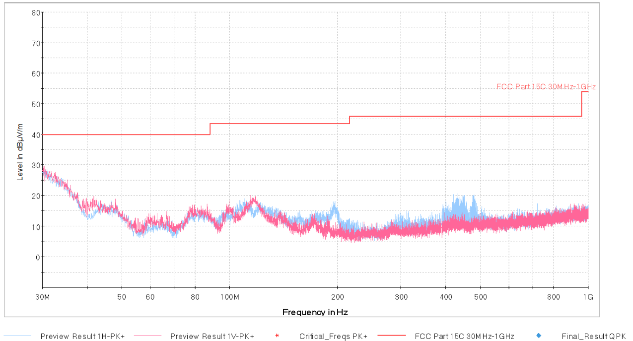
Plot 7-50. Radiated Spurious Plot below 1GHz (Pol. H & V)
