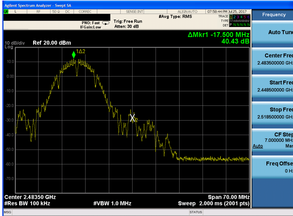
Plot 7-21. Band Edge Plot (802.11b – Ch. 12)
