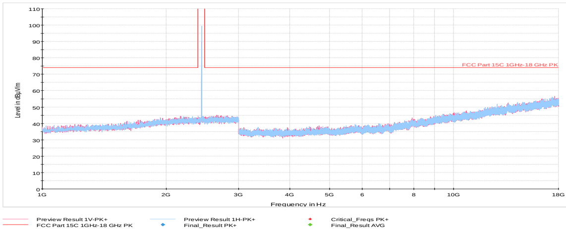
Plot 7-62. Radiated Spurious Plot above 1GHz (BT ePA – Ch. 39, Ant. Pol. H & V)
