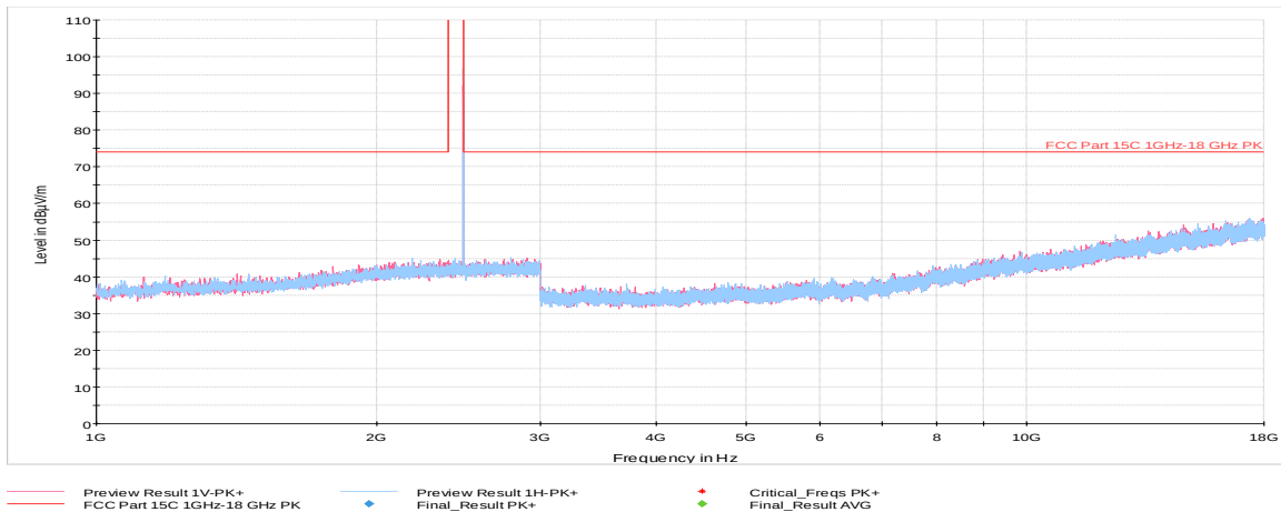
Plot 7-63. Radiated Spurious Plot above 1GHz (BT ePA – Ch. 78, Ant. Pol. H & V)
