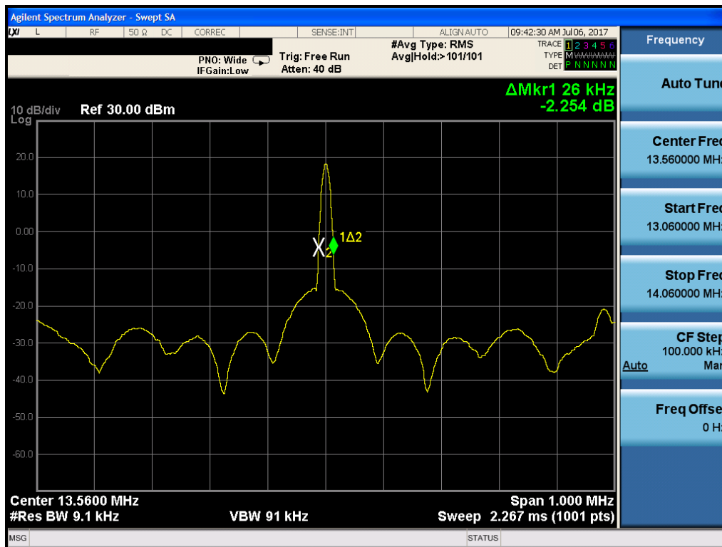
Figure 7-2. 20dB Bandwidth Plot (CE A 848kbps)
