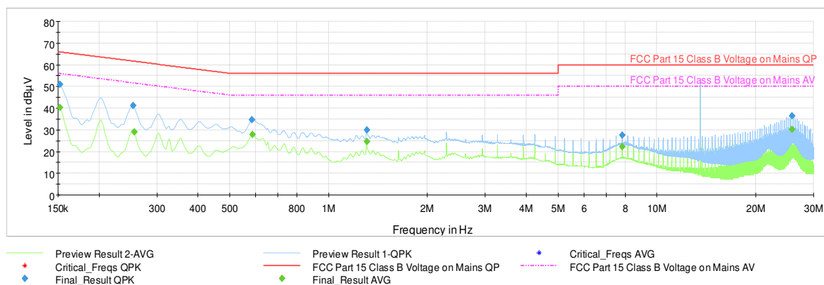
Plot 7-3. Line-Conducted Test Plot (L1)
