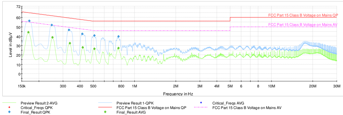
Plot 7-51. Line Conducted Plot with 802.11b (L1)
