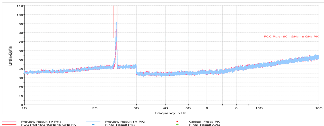
Plot 7-39. Radiated Spurious Plot above 1GHz (802.11b – Ch. 11, Ant. Pol. H & V)
