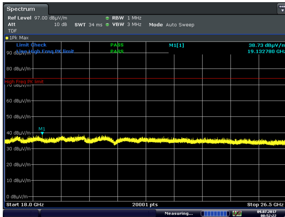
Plot 7-40. Radiated Spurious Plot above 18GHz (802.11b – Ch. 6, Ant. Pol. H)
